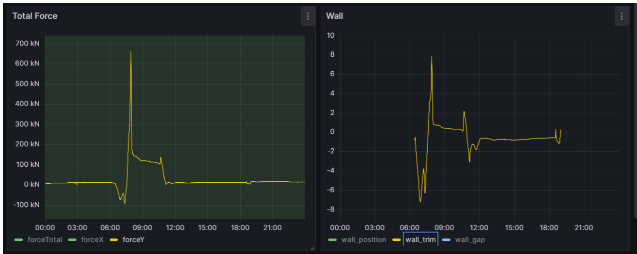
Figure 33: When the tangential force (left panel) is compared to the skewness of the retaining wall during sinking (right panel), one notices a same pattern in the data.
