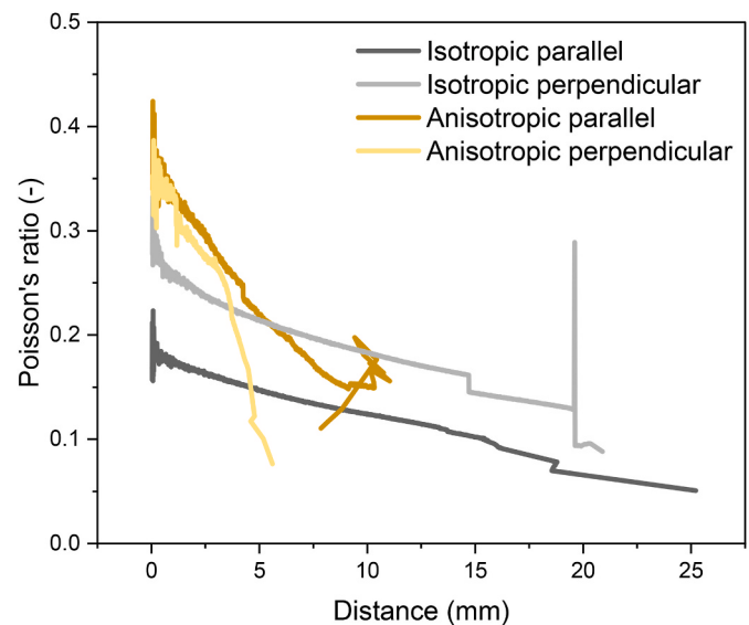
Fig. 12. Dynamic Poisson's ratio over distance during tensile testing for isotropic (grey) and anisotropic (yellow) products parallel (dark) and perpendicular (light) to the shear direction.
