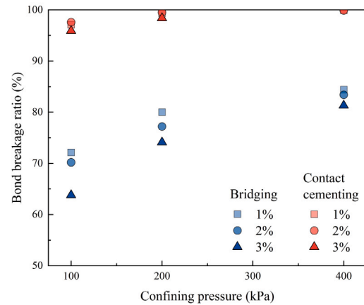
Fig. 16. Evolution of the bond breakage ratio at \varepsilon_1 = 40\% with the confining pressure.
