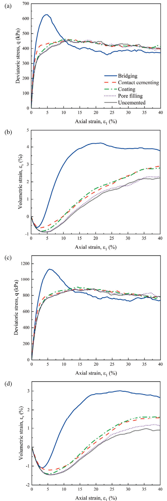
Fig. 5. Effects of the confining pressure on the mechanical response of bio-cemented samples with 1% carbonate content. (a) Stress-strain response and (b) volumetric response upon shearing under a confining pressure of 200 kPa. (c) Stress-strain response and (d) volumetric response upon shearing under a confining pressure of 400 kPa.
