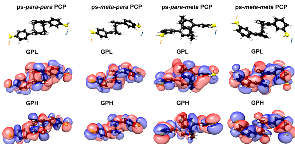
Figure 3.6: HOMO and LUMO molecular frontier orbitals of the ps-para-para -, ps-meta-para -, ps-para-meta -, and ps-meta-meta -PCPs. The anchoring sulfur atoms are marked i and j, respectively. Extended representations also including GPH-1 and GPL+1 for each molecule can be found in the SI3.3 [1].
