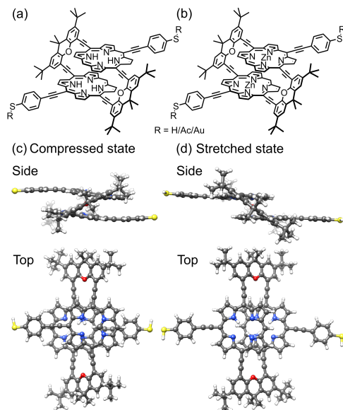
Figure 3.9: Chemical structure of the studied molecules (a) PC1 and (b) ZnPC1. Each of the two central metal Zn ions in ZnPC1 is replaced by two H atoms in PC1. In solution, R represents an acetate (Ac), as synthesized. After in situ deprotection on the gold wire, R is either a hydrogen (H) atom or gold (Au). Side and top views of ball-and-stick representations of calculated (c) compressed and (d) stretched states of PC1 in the gas phase with R = H. Note that compressed and stretched geometries in panels (c) and (d) are both energetic minima.
