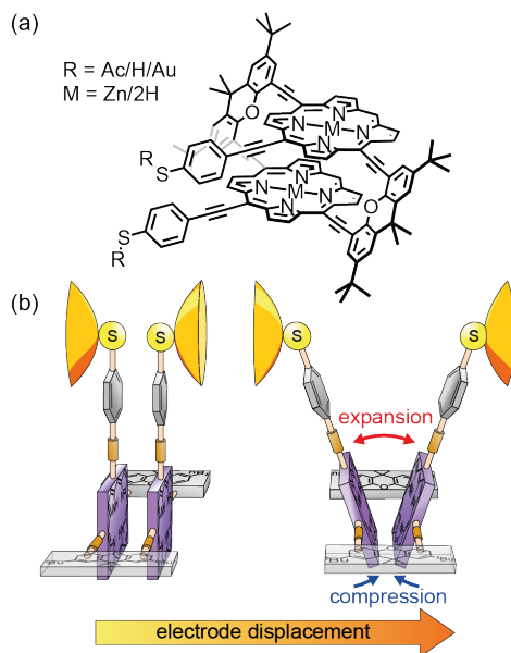
Figure 4.1: (a) Chemical structures of the studied molecules 2HPC2 ( M = 2H ) and ZnPC2 ( M = Zn ). R represents an acetate (Ac) as synthesized or a hydrogen (H) or gold (Au) atom after in-situ deprotection on the gold surface. (b) Cartoon-representation of the hypothesized mechanosensitivity of the intramolecularly \pi -stacked dimer PC2 in an MCBJ experiment.
