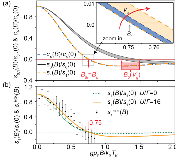
Figure 6.4: (a) Normalized zero-bias thermocurrent slope s_1(B)/s_1(0) and curvature coefficient c_V(B)/c_V(0) vs g\mu_B B/kT_K , for gate voltages 1 \leq V_g = (\epsilon_0 + U/2)/\Gamma \leq 5 in the Kondo regime exhibiting scaling collapse [Anderson model in Fig. 6.1(c) with U/\Gamma = 16 ]. Also shown is the nonuniversal normalized zero-bias thermocurrent s_0(B)/s_0(0) with a sign change at a strongly V_g -dependent B_0 . Inset: c_V(B)/c_V(0) and s_1(B)/s_1(0) in the region around B = B_{th} = B_c \approx 0.75 k_B T_K / g\mu_B , and their V_g -dependence. (b) Least-squares fit of the experimental zero-bias thermocurrent slope s_1^{exp}(B) to the universal curve for s_1(B)/s_1(0) . Error bars denote 1\sigma confidence intervals. A fit to the noninteracting case with U = 0 and \epsilon_0 = -0.1\Gamma (green dotted line) yielded an RMS deviation that was 194% larger than for the Kondo scaling curve. The estimated experimental B_{th} \approx 0.69 k_B T_K / g\mu_B is close to theory ( 0.75 k_B T_K / g\mu_B ).
