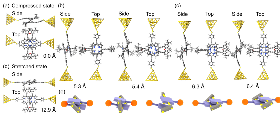
Figure 3.10: PC1 junction geometries in side and top views during the stretching process (a) in the compressed molecular state at an electrode displacement of d \approx 0 Å, (b) at the first and (c) at the second bridge flip at d \approx 5.3 Å and d \approx 6.3 Å, respectively, and (d) in the stretched state at d = 12.9 Å. In the junctions, hydrogen atoms at the thiol termini are removed as compared to the gas phase geometries in Fig. 3.9c and d. (e) Sketch of the evolution of the molecular geometry of PC1 with increasing electrode separation. The molecule is connected to gold tip atoms through terminal sulfur atoms on each side. The electrodes are not displayed in this simplified representation.
