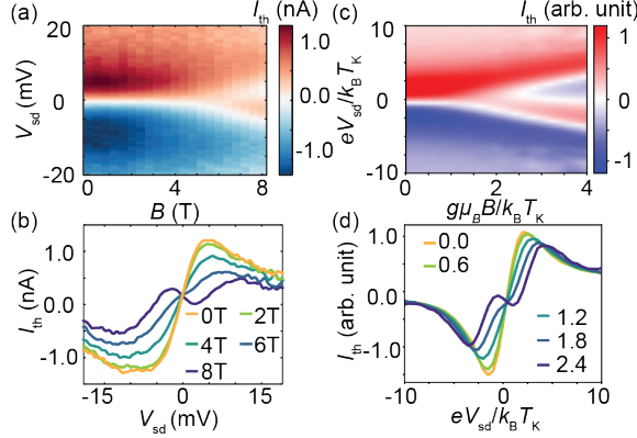
Figure 6.3: (a)-(b) Measured I_{th} , vs V_{sd} at different magnetic fields. (c)-(d) Calculated I_{th} vs V_{sd} at different magnetic fields g\mu_B B / k_B T_K for the Anderson model in Fig. 6.1(c) with V_g = -2.5 , U/\Gamma = 8 , \Delta T/T_K = 0.2 and T/T_K = 0.5 .
