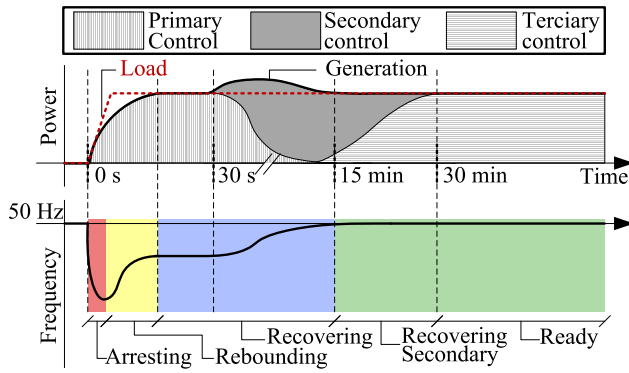
Fig. 1: Sequential activation of primary, secondary and tertiary reserves following a sudden unforeseen event
