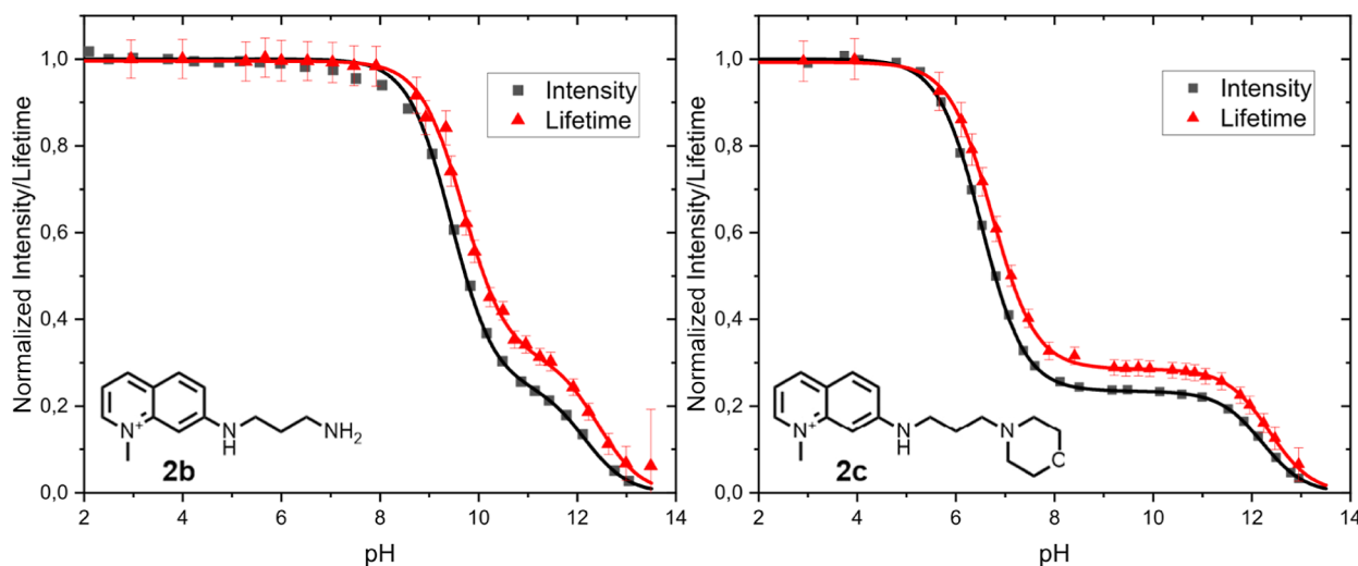
Figure 4. Relative intensity and lifetime vs \text{pH} of probe 2b (left) and probe 2c in water containing 0.1 mM phosphate buffer. The curves around the data points are generated using eq 5, S1, or S5. The error bars in this graph are the standard deviation from the FLIM measurement. See Supporting Information-6 for more information.
