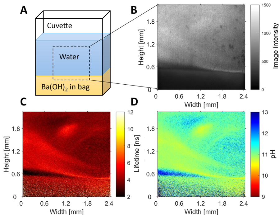
Figure 8. (A) Schematic representation of the experiment: Cuvette with a small paper bag filled with \text{Ba}(\text{OH})_2 powder, on which electrolyte (0.2 M \text{K}_2\text{SO}_4 , 10^{-4} M 2b ) is added using a 5 mL syringe. (B) Light intensity image. (C) Fluorescence lifetime image, calculated from the phase shift from the reference. (D) pH image; lifetime image was converted using the lifetime pH curve from Figure 3.
