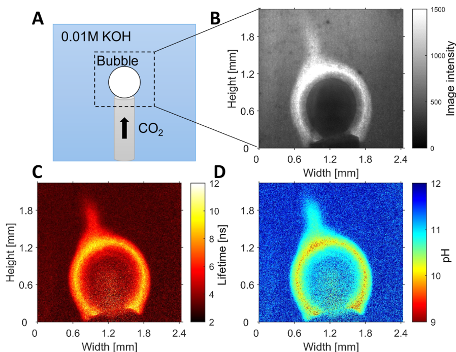
Figure 7. (A) Schematic representation of the experiment: A bubble of \text{CO}_2 pumped in an alkaline (0.01 M KOH, 10^{-4} M 2b ) solution. (B) Light intensity image. (C) Fluorescence lifetime image, calculated from the phase shift from the reference. (D) pH image; lifetime image was converted using the lifetime pH curve from Figure 3.
