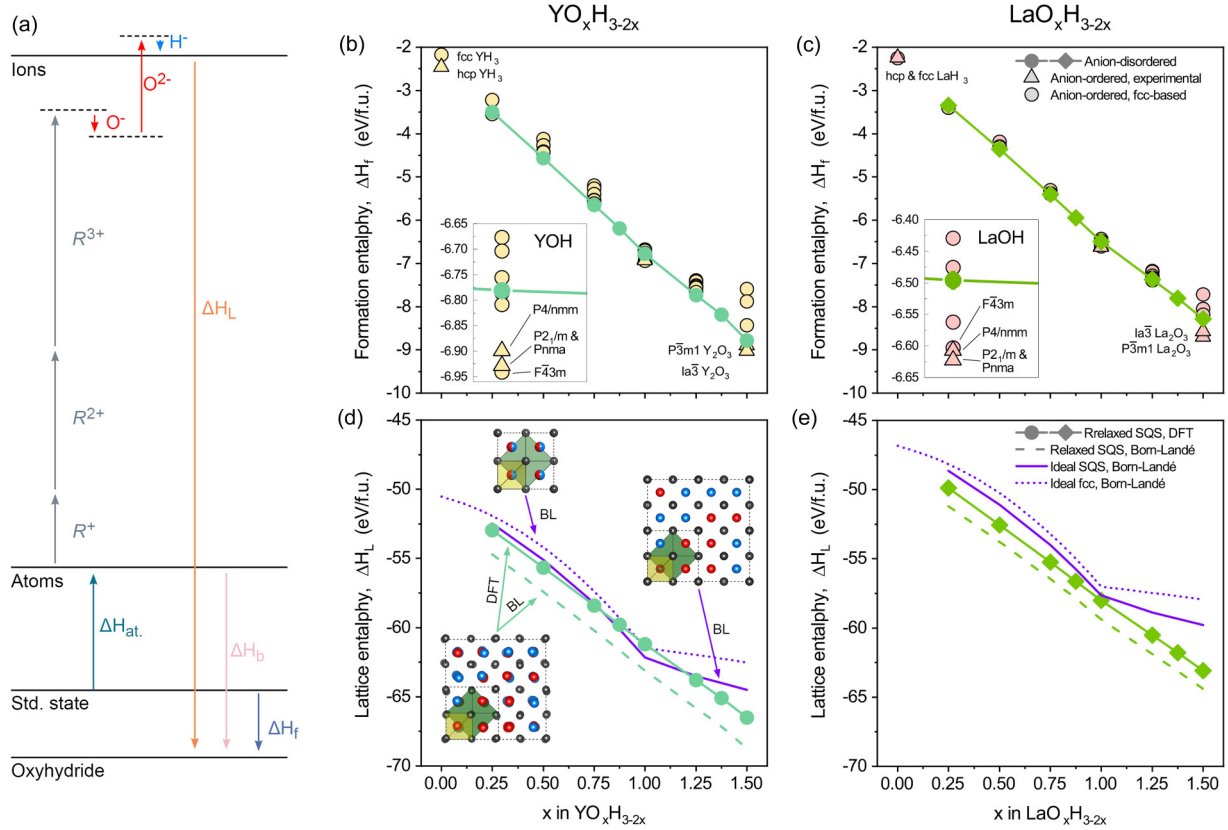
FIG. 4. (a) Born-Haber cycle of R oxyhydride. The arrows are at scale for the 1:1:1 composition and indicate: Atomization energy ( \Delta H_{at} ), R ionization energies, O and H electron affinities, oxyhydride lattice energy ( \Delta H_L ), binding energy ( \Delta H_b ), and formation energy ( \Delta H_f ). [(b), (c)] Influence of O:H ratio on the formation energy of Y and La oxyhydrides, respectively. The insets focus on the stoichiometric 1:1:1 composition. [(d), (e)] Influence of O:H ratio on the lattice energy of Y and La anion-disordered oxyhydrides, respectively. For x \leq 1 , the (negative) lattice energy increases mainly due to a shift of charge from the less-stable octahedral to the more-stable tetrahedral anion sites. For x > 1 , further stabilization results from a larger freedom for structural distortion related to the presence of empty tetrahedral sites. For comparison, the lattice energy evaluated with the Born-Landé equation is also reported for three different structural models of increasing resemblance to the real material: (i) idealized anion-disordered model based on Fm\bar{3}m symmetry (dotted lines), (ii) nonrelaxed SQS structures (solid lines), and (iii) relaxed SQS structures (dashed lines).
