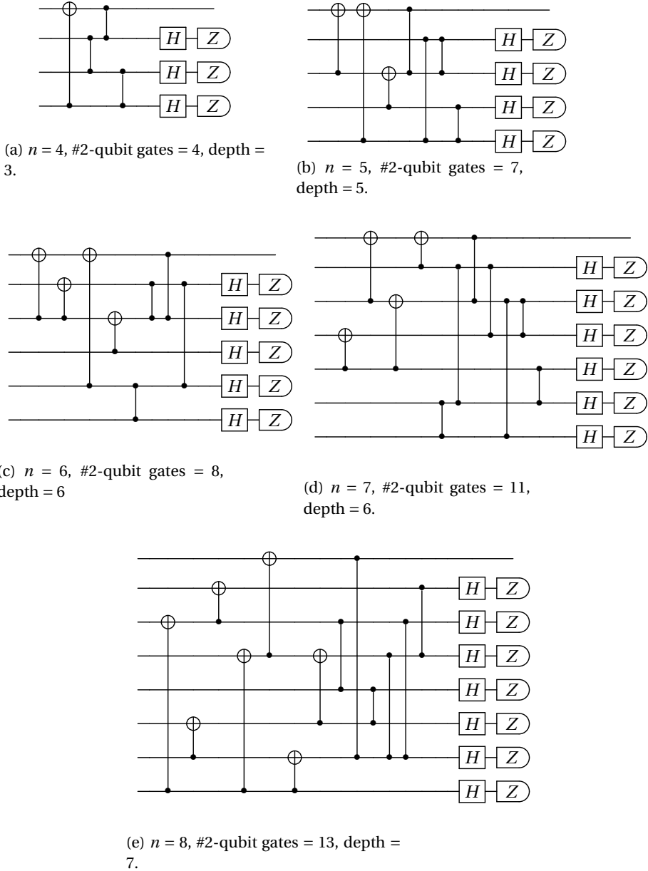
Figure 5.8: Circuits that achieve the maximum fidelity for n . These circuits are applied by both Alice and Bob, after which they measure the last n - 1 qubits, and communicate their outcomes to each other. When the outcomes for all individual qubit pairs are correlated, the distillation protocol was deemed successful.
