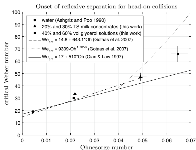
Fig. 10 Onset for reflexive separation regime for head-on collisions ( B = 0 )
