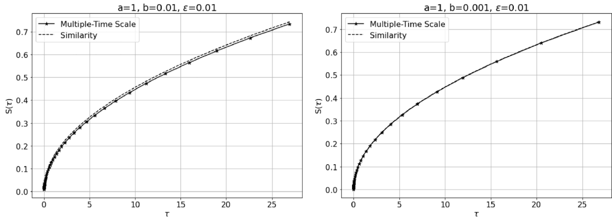
Fig. 4. Moving boundary profile for small values of b .
