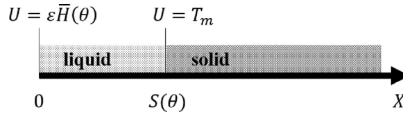
Fig. 1. Melting process of a semi-infinite ice sheet due to the temperature \varepsilon\bar{H}(\theta) at X = 0 .
