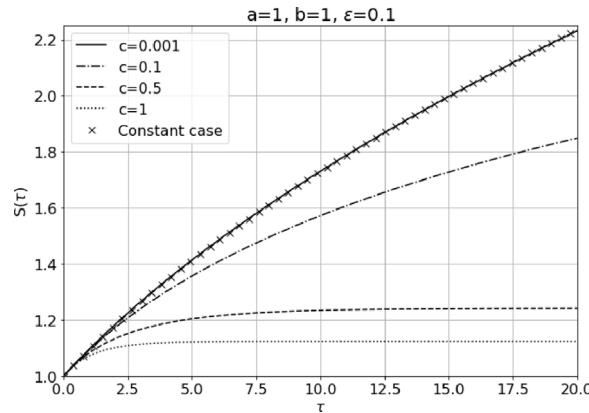
Fig. 7. The moving boundary profile in case of a decaying temperature at the fixed endpoint for different values of the decaying rate c .
