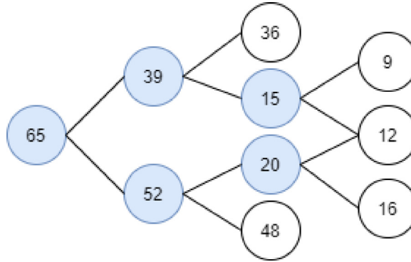
Fig. 2. Illustration of Pythagorean branching that occurs for the case with n = 65 as head of the chain.
