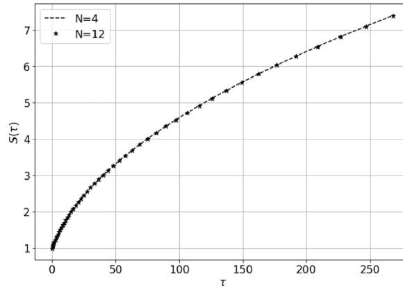
Fig. 3. Comparison of the approximations of the interface S(\tau) for N = 4 and for N = 12 .
