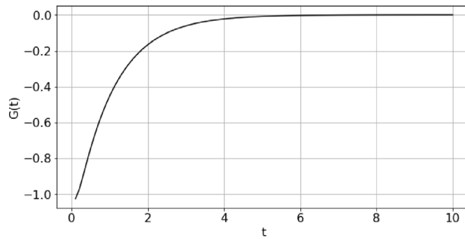
Fig. 8. Plot of G(t) in time ( c = 1 ).
