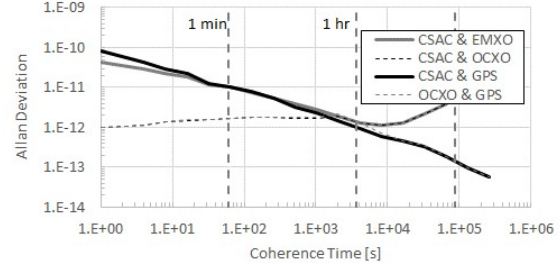
Fig. 3 Allan deviations for selected 2-component heterogeneous clock systems as a function of coherence time.
