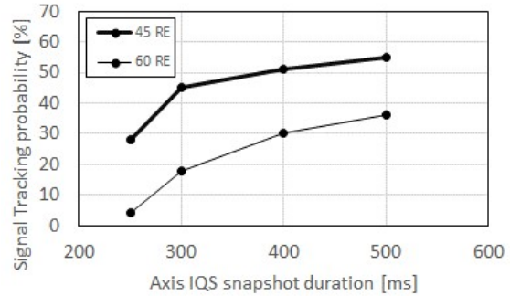
Fig. 7 Probability for tracking GNSS signals w.r.t. I-Q samples (IQS), parametrized with Spacecraft-Earth distances in units of Earth radius (RE). Values taken from [Nardin et al. 2023].
