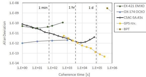
Fig. 2 Allan deviation for various clock components as a function of coherence time (data taken from [van Buren 2020], [Lutwak 2011] and [Lombardi et al. 2001]). BPT stands for Binary Pulsar Timing.
