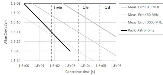
Fig. 1 Allan deviations of phase measurement errors for various frequencies and the scientific requirement from a specific radio astronomy application (Relations and data from [Rajan et al. 2013]).
