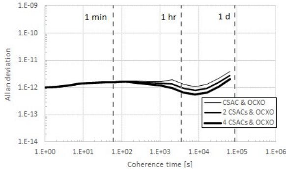
Fig. 5 Allan deviation for the CSAC – OCXO system with multiple CSAC units.
