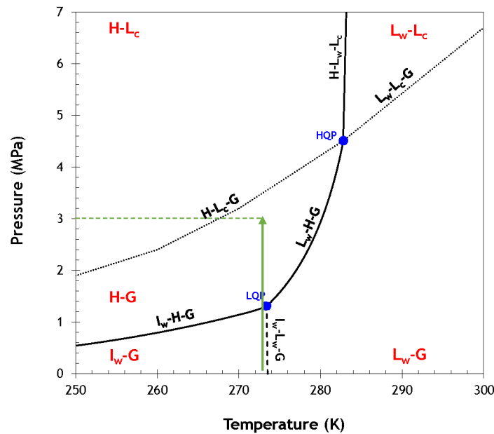
Figure 2—Three-phase diagram of the CO 2 -water mixture. The symbols I_w , L_c , L_w , H , and G represent ice water, liquid CO 2 , liquid water, hydrate, and gas, respectively. HQP and LQP refer to high ( L_wHL_cG ) and low ( I_wHL_wG ) quadruple points. The smooth line represent the three-phase equilibrium line, the dotted line indicate the CO 2 condensed line, and the dashed line is ice line.
