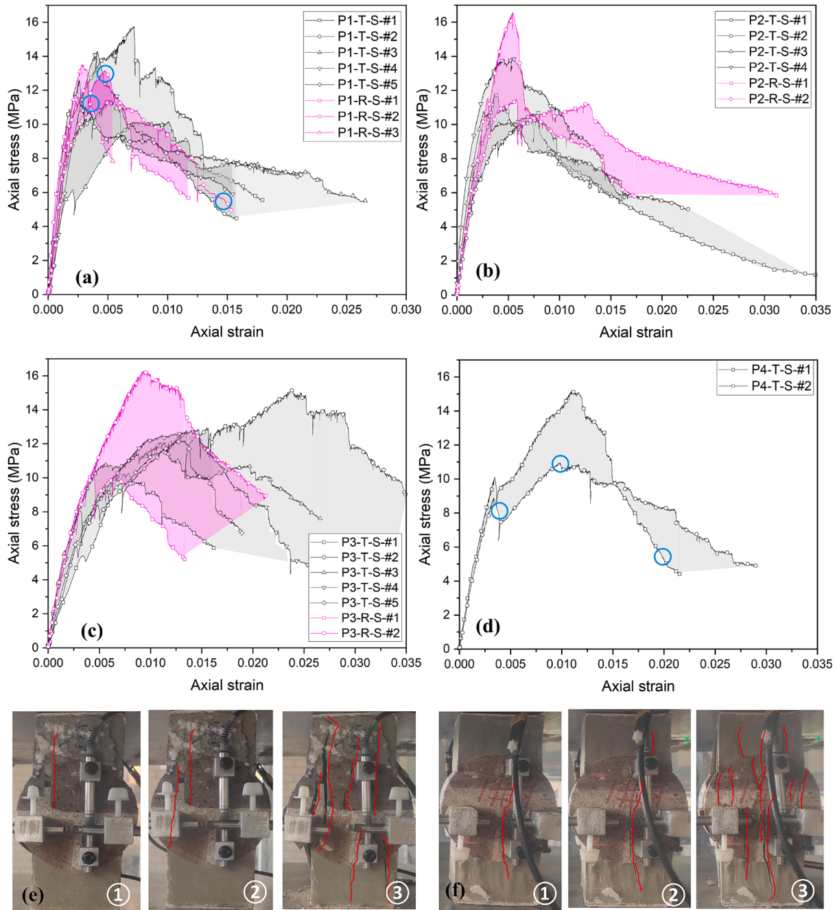
Fig. 3. Axial stress versus axial strain under compression for single-wythe cores extracted from: P1(a), P2(b), P3(c) and P4(d); the evolution of crack pattern for core P1-R-S-#2 (e) and P4-T-S-#2 (f).
