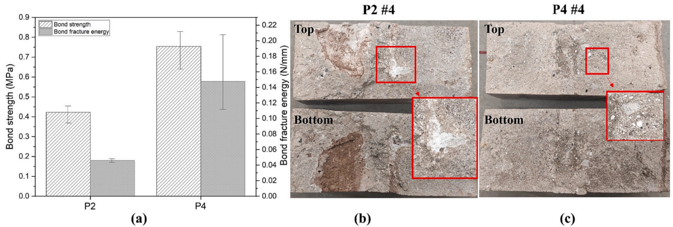
Fig. 13. Mean values of bond strength and bond fracture energy for couples extracted from P2 and P4 (a); Crack surface of the sample from P2 (b); Crack surface of the sample from P4 (c).
