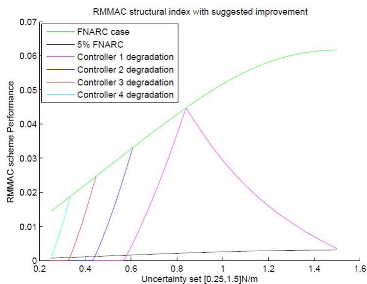
Figure 16. Modified RMMAC scheme with uncertainty of [0.25, 1.5]N/m .
