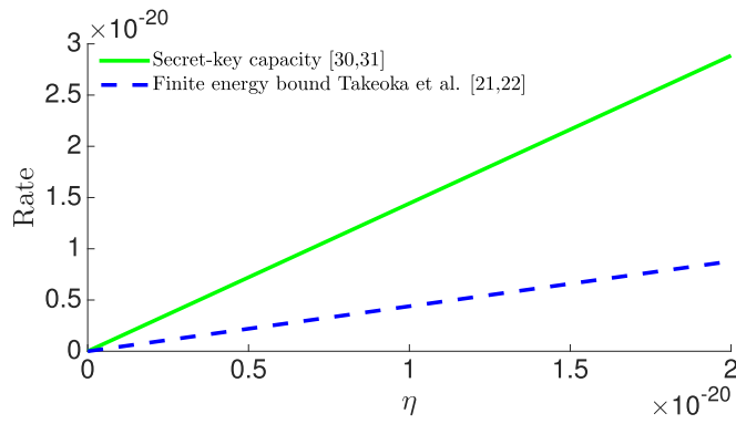
Figure 6. Bound for the pure-loss channel with an average photon number of 0.1 and the secret key capacity [30, 31] as a function of \eta . The new bound in this paper coincides with the finite-energy variant of the bound by Takeoka et al , see [21, 22]. The loss parameter \eta ranges from 0 to 2 \times 10^{-20} , which is the range of expected losses for transmissions across fibers with length \approx 1000 km with an attenuation length of 22 km [18].
