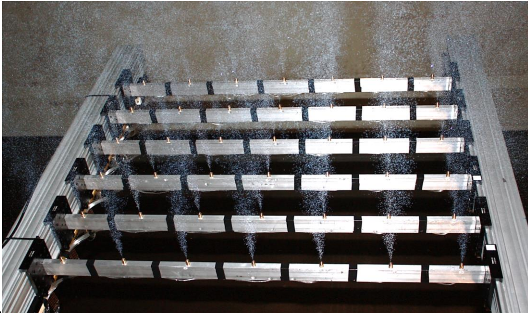
Figure 2. NLR's HFSB 42-bubble generators seeding rake.
