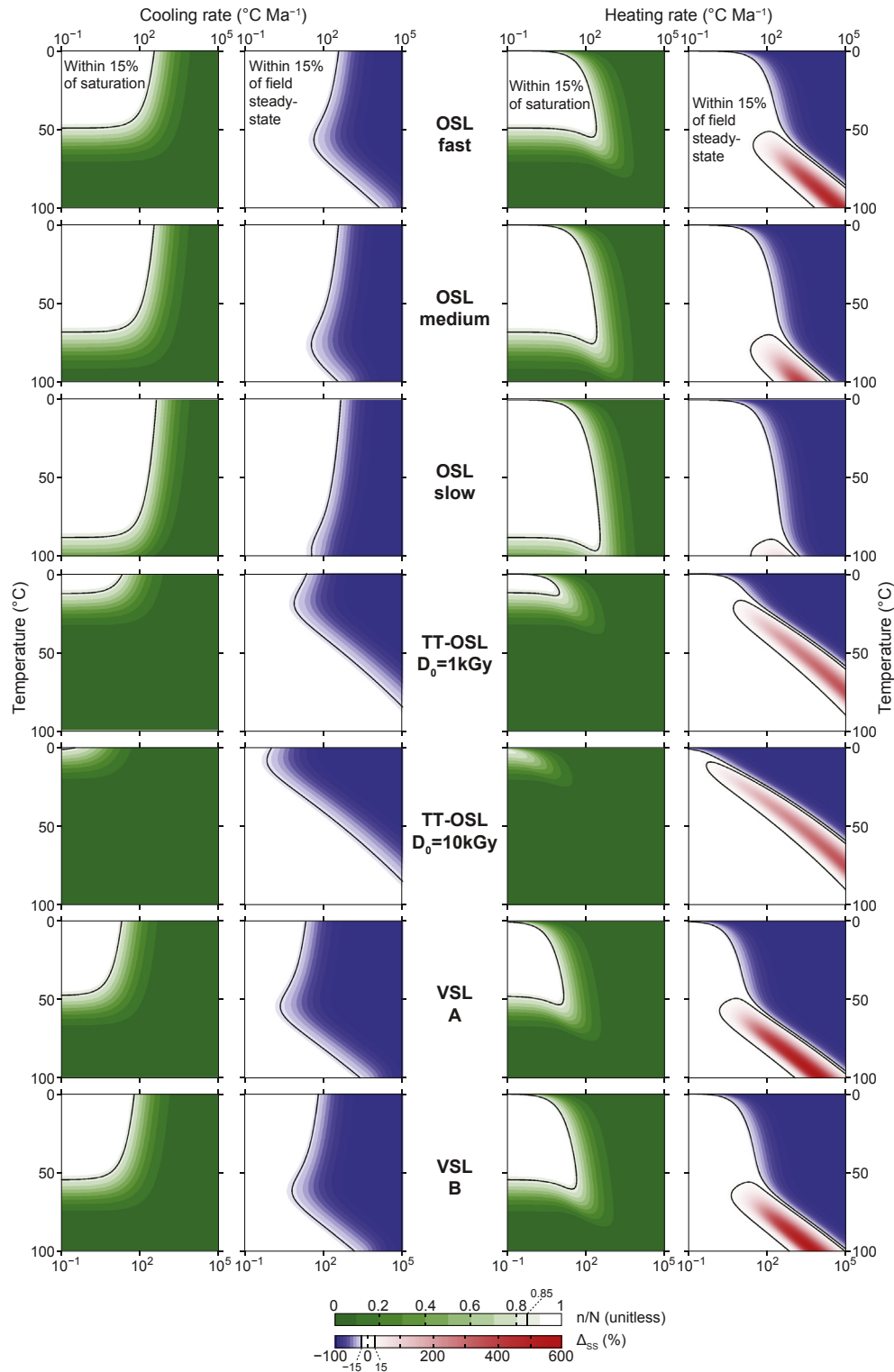
Fig. 4. Comparison of trap filling (columns 1 and 3) and relative disequilibrium conditions (columns 2 and 4) as explained in Fig. 3, for various OSL signals encountered in the literature (Table 2) and subjected to linear cooling (columns 1–2) and heating (columns 3–4) scenarios.
