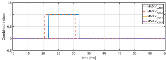
(b) Combined indices of critical relays
