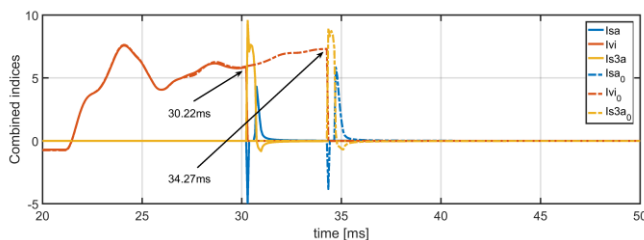
Fig. 13. Currents of DCCB1 with different delays
