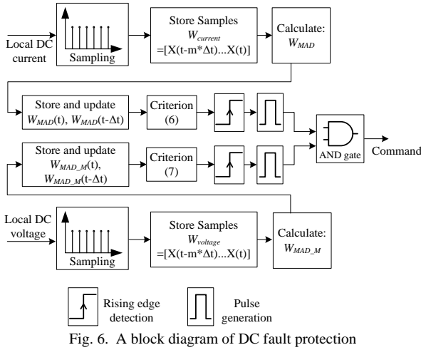
Fig. 6. A block diagram of DC fault protection
