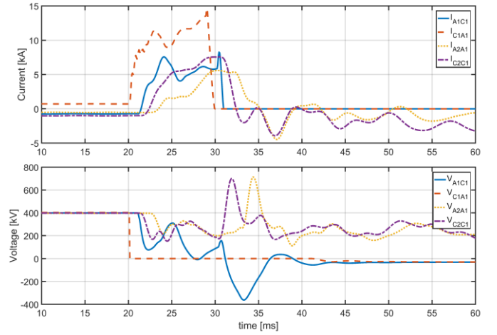
Fig. 8. Currents and voltages measured by criterial relays
