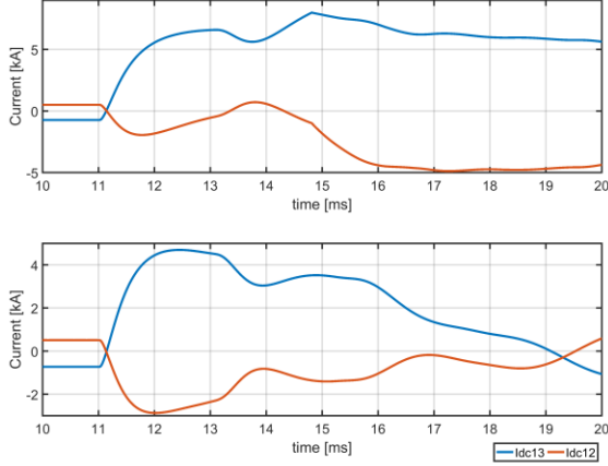
Fig. 2. Neighboring currents due to a fault on Line13. Upper plot: pole-to-pole fault. Bottom plot: pole-to-ground fault.
