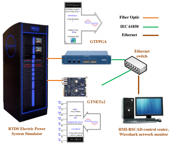
Fig. 7. Real time simulation platform based on RTDS and IEC 61850 based ICT infrastructure
