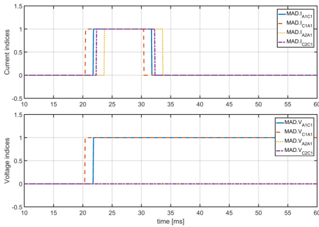
(a) Current and voltage indices of critical relays
