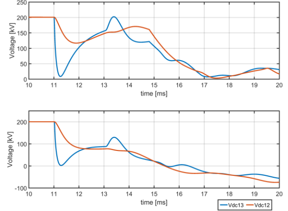
Fig. 3. Responses of voltage at the end of line to fault on Line13. Upper plot: pole-to-pole fault. Bottom plot: pole-to-ground fault.
