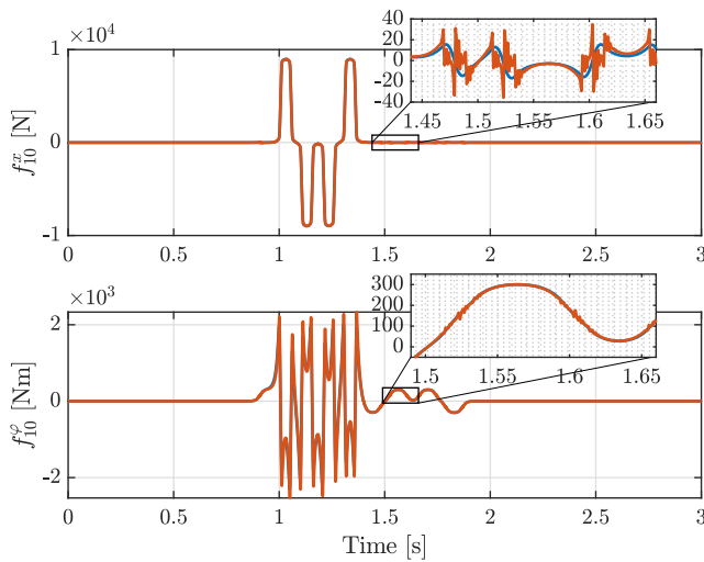
Fig. 7. Feedforward signals in trial j = 10 of the RBF algorithm for SISO systems (—) and the developed MIMO RBF approach (—). Noteworthy, in contrast to the RBF algorithm for SISO systems, the feedforward signal of the developed approach compensates for dynamics that are seen in Fig. 6.
