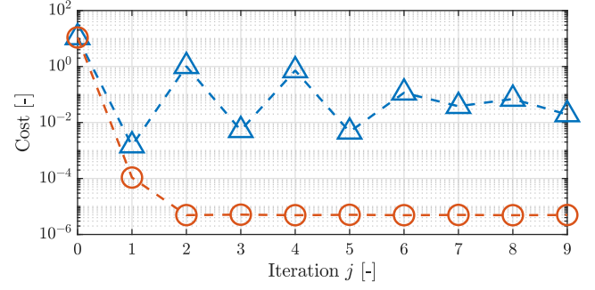
Fig. 5. Cost per iteration j for the RBF algorithm for SISO systems ( \triangle ) and the developed MIMO RBF approach ( \circ ). Clearly, the RBF algorithm for SISO systems does not necessarily converge.
