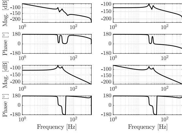
Fig. 4. Bode diagram of the P(z) used in simulation and ILC design. Clearly, the MIMO system has substantial interaction between axis and is not symmetric.
