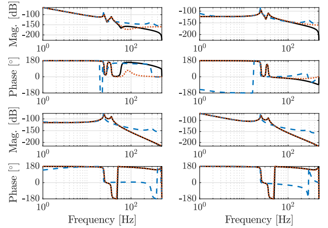
Fig. 6. Bode diagram of the plant P(z) ( \longrightarrow ) and of the inverse feedforward filters F^{-1}(z, \theta_{10}) in trial j = 10 achieved with the RBF algorithm for SISO systems ( \dashrightarrow ) and the developed approach ( \cdots ). The feedforward filter of the developed approach fits the resonance and anti-resonance peaks of the plant significantly better, allowing enhanced performance.
