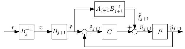
Fig. 3. Closed-loop RBF control scheme of Fig. 2(c) rewritten to recover the RBF algorithm using SK-iterations for commutative systems.
