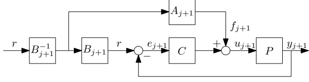
(b) Rewritten closed-loop RBF control scheme for iteration j + 1 .
