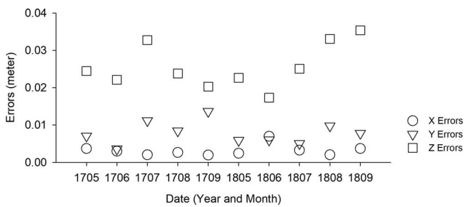
Figure 4. The LIDAR data errors in the plan space (circles and triangles) and vertical direction (squares).
