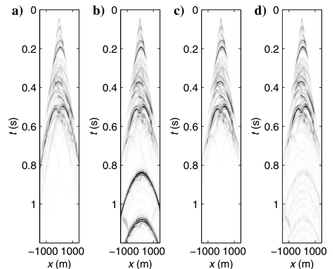
Figure 5. (a) Reflection response from below with a source at \mathbf{x} = 0 on \partial\mathcal{V}_j and receivers on the same level, computed in the reference medium. A similar reflection response, retrieved by single-sided redatuming of focusing functions (i.e., inversion of equation 23). Similar reflection responses, retrieved by target-enclosed redatuming of the (c) Green's functions (i.e., inversion of equation 15) and (d) focusing functions (i.e., inversion of equation 24). All figure parts have been normalized with respect to their maximum value.
