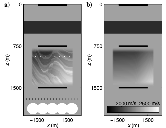
Figure 2. (a) Propagation velocity in the physical medium (the color bar is shown in [b]). (b) Macro velocity model with color bar. The black lines at z = 0 , 750 , and 1500 m indicate arrays at boundaries \mathcal{S}_a , \partial\mathcal{V}_i , and \partial\mathcal{V}_j , respectively. The target zone is defined as the part of the medium where z \in [750, 1500] m.
