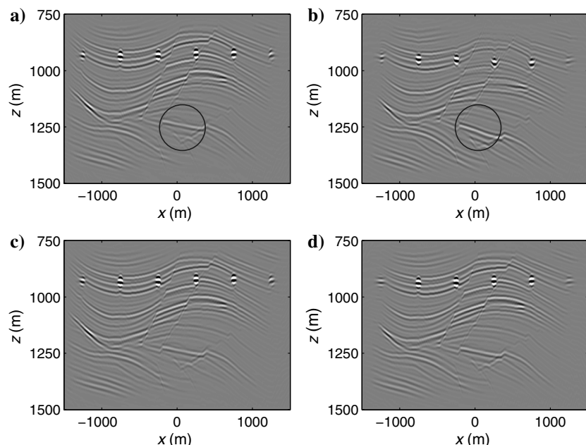
Figure 6. Linear images of the target from (a) above and (b) below after redatuming with kinematically correct focusing functions. The black circles highlight a reflector that is discussed in the main text. Linear image of the target from (c) above and (d) below after redatuming with approximate focusing functions. Here, linear imaging is defined as imaging of primary reflections in the macro model. The images from below have been multiplied with -1 such that all images have the same polarity.
