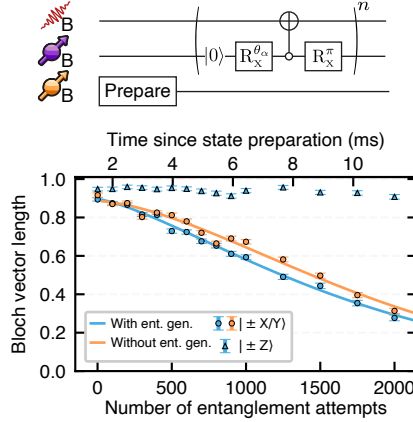
Figure 4.3: Memory qubit coherence under network activity. (Top) Circuit diagram displaying the experimental sequence, where n is the number of entanglement attempts. (Bottom) Blue represents the measured Bloch vector length of memory qubit eigenstates (triangles) and superposition states (circles) versus entanglement attempts, for \alpha = 0.05 . Orange represents measured superposition decay versus time in the absence of entanglement attempts. Solid lines are fits, yielding decay constants of N_{1/e} = 1843 \pm 32 ( 2042 \pm 36 ) with (without) entanglement generation attempts (see Table 4.5 and Section 4.6 for additional details).
