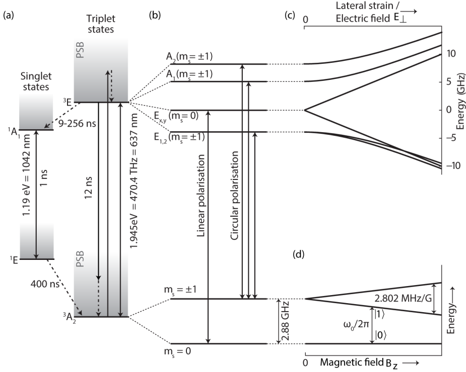
Figure 2.3: Electronic energy level structure of \text{NV}^- Adapted from Bernien, Pfaff, Kalb [3, 4, 17] (a) The spin-triplet ground states ^3A_2 and excited states ^3E are optically connected, as well as the spin-singlet ground state ^1E and excited state ^1A_1 . Excitation and emission can happen resonantly or off-resonantly via vibronic states, the phonon side band (PSB, shaded blocks). A spin-flipping channel is opened via an intersystem crossing, the ^3E states can decay to ^1A_1 , with a rate dependent on the exact state (9 – 256ns [16]). The decay from the ^1E state to the ^3A_2 states is temperature dependent and at cryogenic temperatures \approx 400\text{ns} [16]. (b) Due to spin-orbit interactions the ^3A_2 ground state is split into two levels. The ^3E excited states are split because of spin-spin and spin-orbit couplings. These couplings result in two doubly degenerate states E_{x,y} and E_{1,2} . At cryogenic temperatures, the optical transitions can be addressed state selectively. (c) Strain or electric fields can distort the crystalline symmetry of the defect and shift the energy levels of the excited state. (d) An external magnetic field along the NV crystal axis, B_z , splits the energy levels of the |m_s = \pm 1\rangle spin states due to the Zeeman effect.
