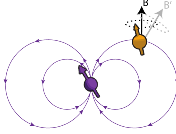
Figure 2.8: Interaction between the communication qubit and a nearby ^{13}\text{C} nuclear spin. Adapted from Cramer [34]. When the communication qubit (purple spin) is in |m_s = 0\rangle , the precession of the nuclear spin (orange spin) is given by the external magnetic field B . When the communication qubit is in |m_s = \pm 1\rangle , the local magnetic field of the nuclear spin is altered, as a consequence the nuclear spin will precess with a different frequency around a tilted axis.
