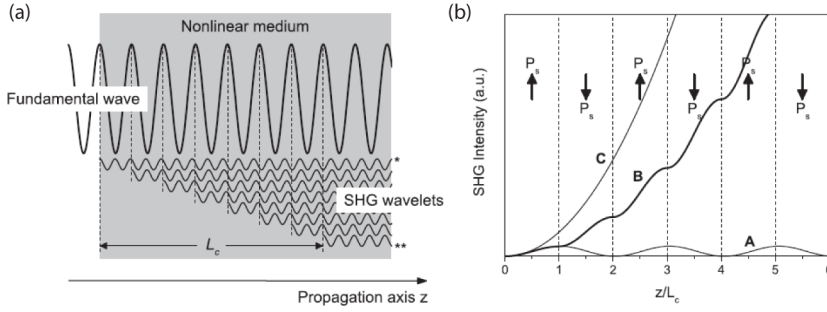
Figure 2.10: Quasi-phase matching Adapted from Zaske [40]. (a) Illustration of the second-harmonic generation (SHG) process. Over the whole length of the non-linear medium the conversion process converts the fundamental wave to a second-harmonic (SH) wave. Due to dispersion in the medium, the fundamental and the SH wavelets travel with different velocities. After the coherence length L_c , newly generated SH wavelets destructively interfere with SH wavelets created at L = 0 . (b) As a consequence, the conversion efficiency will alternate with a period of L_c and in general be small (A in the diagram). In the case of quasi-phase matching the sign of the induced polarization is changed every L_c by electrical poling and the conversion efficiency will increase of the entire length of the crystal (B in the diagram). For comparison, if we would be able to achieve perfect phase matching, the conversion efficiency would increase as curve C in the diagram.
