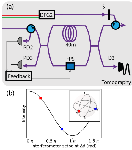
Figure 3.3: (a) Polarization-maintaining fiber-based imbalanced interferometer used for the photon state read-out in X and Y bases. The frequency-converted single photons are directed into the interferometer. One output port of the interferometer is connected to a superconducting nanowire detector (detector D3). Every second the phase of the interferometer is stabilized. Classical frequency-converted light created by a second DFG setup (DFG2) is sent into the interferometer via a shutter S and a circulator. Light intensities measured by photodiodes PD2 and PD3 are used to generate a feedback signal to the fiber piezo stretcher (FPS) to maintain the target phase \Delta\phi . (b) Bloch sphere with the selected photon qubit readout bases indicated on it, and the corresponding phase set points of the imbalanced interferometer.
