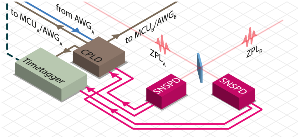
Figure 2.14: Schematic diagram of the equipment used to herald remote entanglement Zero-phonon line photons from two setups are interfered on the central beam splitter. The output ports of the beam splitter are connected to two superconducting nanowire single photon detectors (SNSPD). The detection times of the photons are recorded using a timetagger. A complex programmable logic device (CPLD) is programmed to determine whether a photon detection is an heralding event based on input signals from the arbitrary waveform generator (AWG) of node A. When entanglement is heralded the CPLD informs the microcontrollers (MCU) and the AWGs of both nodes.
