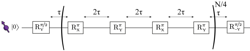
Figure 2.7: Communication qubit decoupling sequence Any superposition state encoded on the communication qubit starts to dephase as soon as it is created (by the R_Y^{\pi/2} -rotation the diagram), because of undesired interactions with the surrounding spin bath. To preserve superposition or entangled states, we decouple the communication qubit from the bath using sequence of N gates. In these decoupling sequences \pi -pulses are equally spaced in time, 2\tau apart, to cancel dephasing errors caused by the bath. In the diagram an XY4 sequence is shown as an example. Throughout the thesis we make use of XY4 as well as XY8 sequences, as these sequences mitigate the effect of pulse errors [32].
