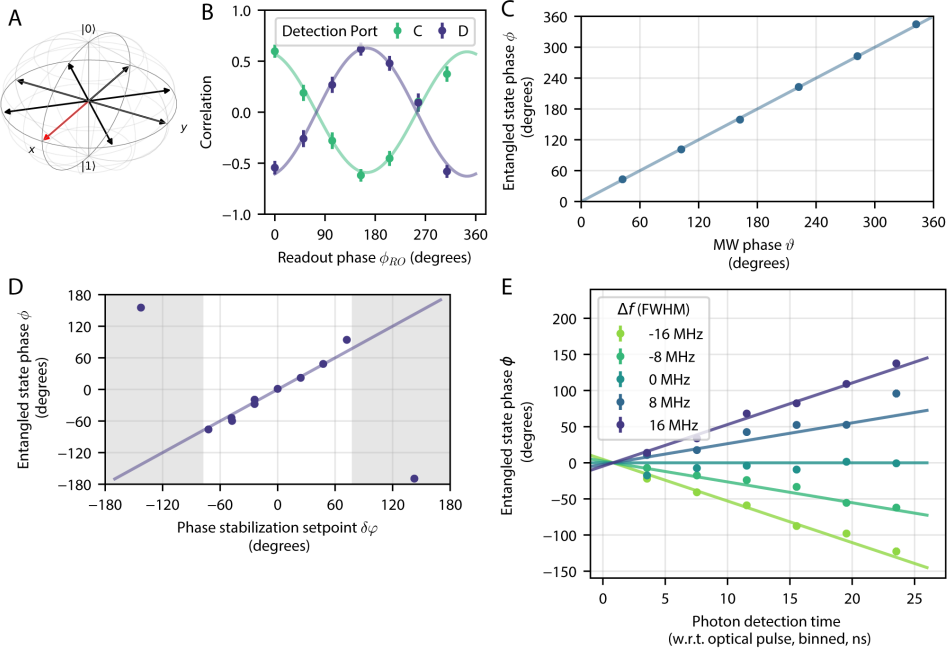
Figure 6.4: Entangled state phase. (A) We determine the entangled state phase by measuring along the +X axis on setup B (red arrow), while sweeping the measurement axis of setup C over the equator plane of the Bloch sphere (black arrows). In this way we obtain oscillating correlations between the measurement outcomes, as shown in (B), for states heralded by detector C (turquoise circles) and D (purple circles). We jointly fit the data for the two detectors to extract \phi , the phase offset with respect to a cosine. (C) The entangled state phase \phi as a function of the phase of the microwave (MW) pulse we use to create the initial superposition state (see Eq. (6.2)). Here we fix \vartheta_C = 0 and sweep \vartheta_B . Due to a small difference of the stabilized path compared to the path of the excitation pulses and the single photons, there is a nonzero phase offset [20]. We fit the measured phase values with a line with slope 1 and subtract the fitted offset. The solid line represents the expected behavior. (D) The entangled state phase as a function of the optical phase stabilization set point. Again we account for the phase offset due to path difference and shows the expected response (solid line). (E) The entangled state phase as function of the detection time of the photon for different frequency offsets between the setups. The photon detection times are binned in bins of 4 ns, and the x value represents the middle of the bin. The time scale is with respect to the highest intensity point of the optical pulse. The solid lines are a joint fit the data with the zero point crossing x_0 as the only free parameter. The fit gives x_0 = (0.8 \pm 0.3) ns. The error bars of the data plotted in (C), (D) and (E) are smaller than the symbol size.
