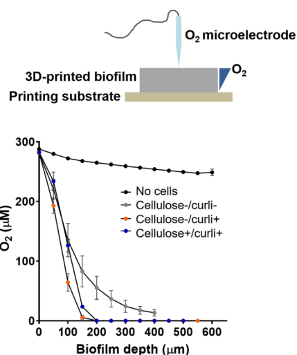
Figure 4. Oxygen profiles of four-layered 3D-printed biofilms revealing the presence of zero- O_2 zones in the bottom layers. An oxygen microelectrode was used to profile the oxygen concentration at different depths in 3D-printed E. coli . The deepest O_2 measurement coincides with the bottommost point of the 3D print at the interface with the supportive media such that the thickness of 3D prints can be compared with this method.
