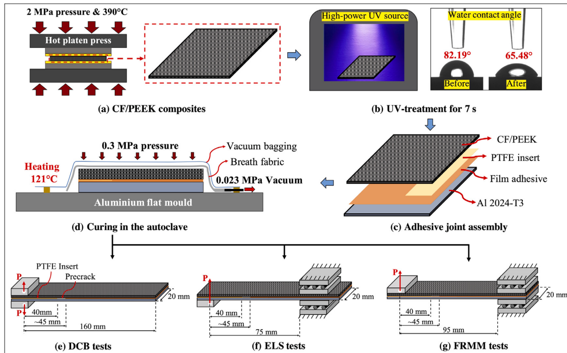
Fig. 1. Illustrations for the sample preparation and fracture tests of the adhesive joints.
