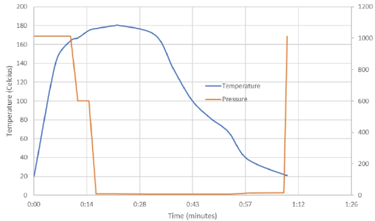
Figure 4: Pressure and temperature development (2)
