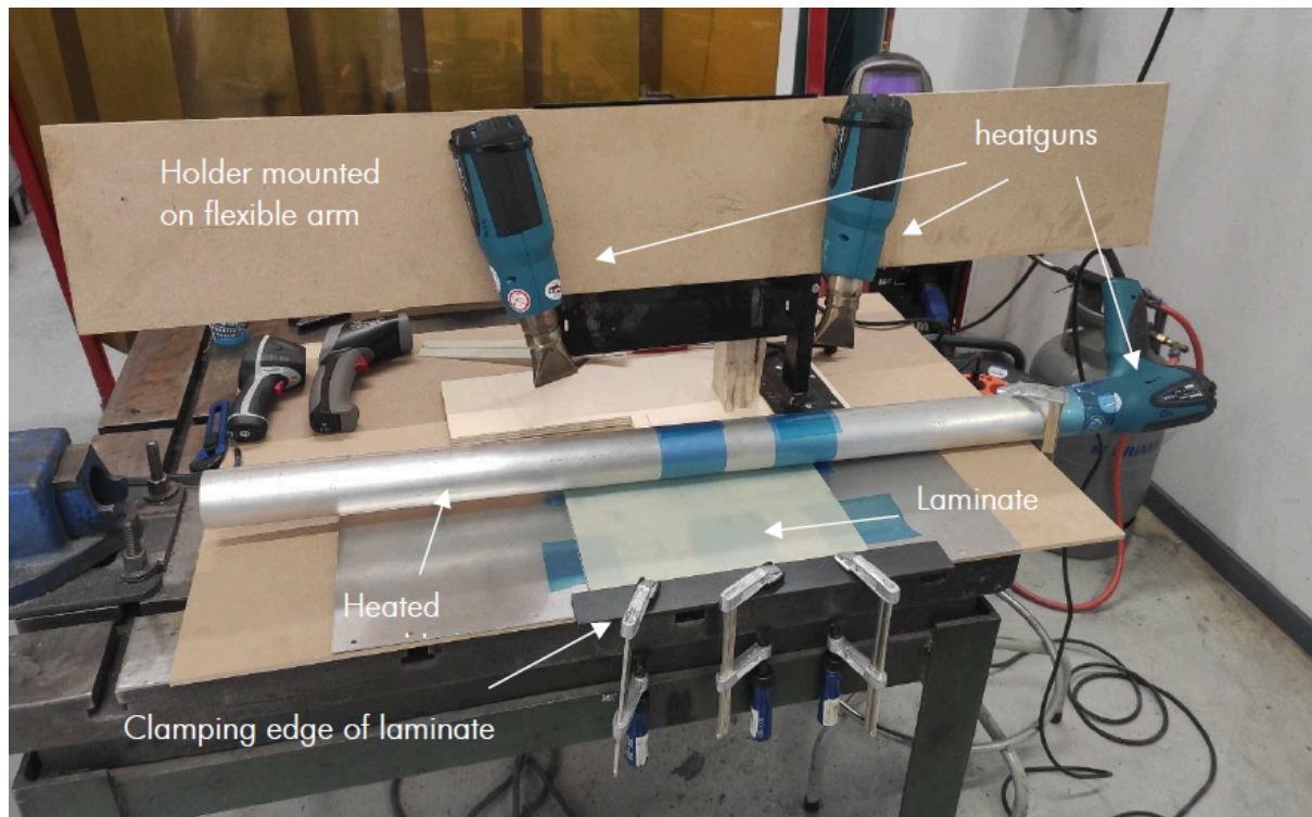
Figure 7: Setup of reshaping experiment 4
