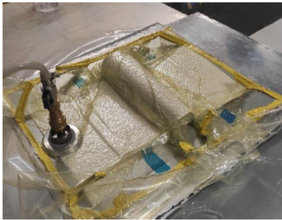
Figure 1: Reshaping experiment 1, formed
