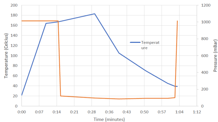
Figure 6: Pressure and temperature development (3)
