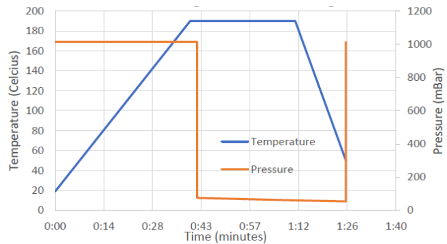
Figure 2: Pressure and temperature development (1)
