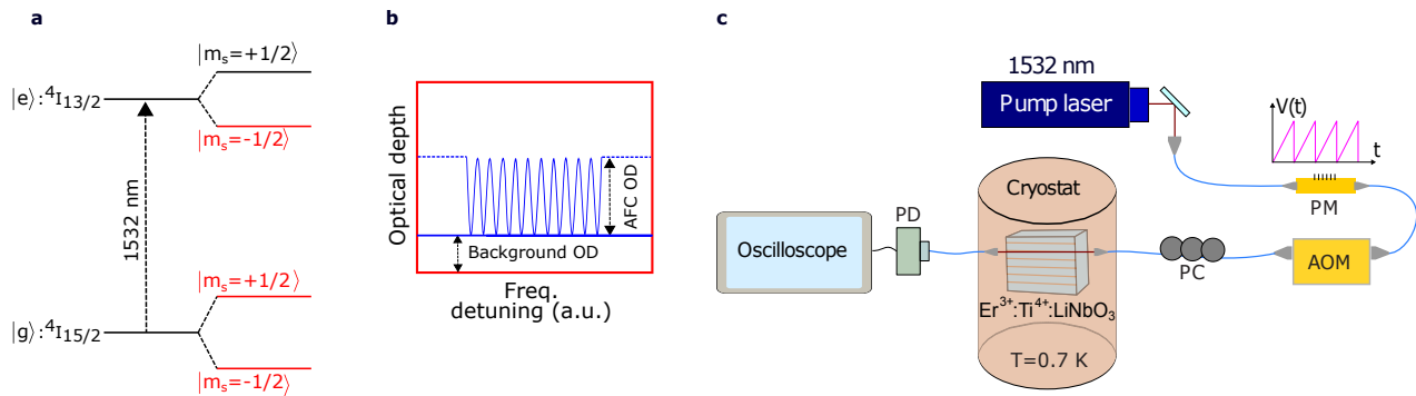
Fig. 1. a. Simplified energy level structure of the {}^4I_{15/2} \leftrightarrow {}^4I_{13/2} transition of \text{Er}^{3+} . Excited and ground levels are indicated with |e\rangle and |g\rangle , respectively, and electronic Zeeman sub-levels with |m_s = \pm 1/2\rangle . To create an atomic frequency comb (a periodic modulation of the frequency-dependent optical depth into equally-spaced narrow peaks), persistent spectral holes are created (burned) by pumping all undesired population into shelving levels, e.g. |g, m_s = +1/2\rangle . b. An example of an AFC, showing the resulting spectral population grating. c. Experimental setup. Continuous-wave light at 1532 nm wavelength is directed through a phase-modulator (PM) and an acousto-optic modulator (AOM), which allow frequency and intensity modulation. After passing a polarization controller (PC), the light creates spectral holes and AFC structures in the erbium-doped lithium niobate waveguide, and furthermore allows probing previously created structures with the help of a photo-detector (PD) and an oscilloscope. The PM is driven by a serrrodyne voltage V(t) modulation similar to that depicted in the plot.
