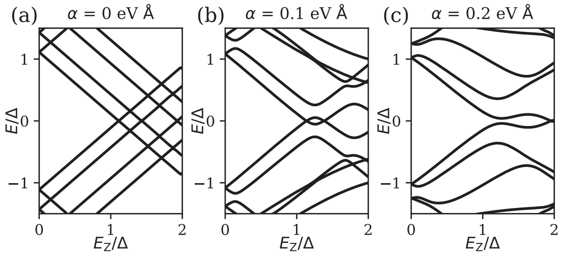
Figure 12. Calculated low energy spectrum of the finite size nanowire as a function of Zeeman energy for different values of \alpha . Values calculated for V_{\text{Gate}} = -0.536 V, which is also used in main text figure 4(d). All energy scales are in units of the superconducting gap \Delta .
