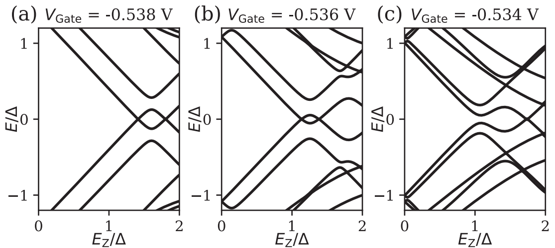
Figure 13. Calculated low energy spectrum of the finite size nanowire as a function of Zeeman energy for different values of V_{\text{Gate}} . Values calculated \alpha = 0.1 eV Å, energy scales in units of \Delta .
