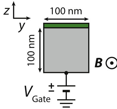
Figure 11. Schematic cross-section of the geometry used to simulate the finite nanowire system. A potential V_{\text{Gate}} is applied to the bottom facet, while the potential at the top facet is fixed by the work function difference between the two materials. The magnetic field is applied in the x -direction, along length of the nanowire.
