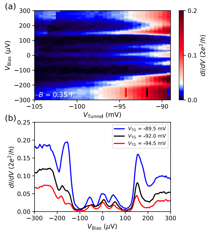
Figure J1. (a) dI/dV measured in device A as a function of V_{\text{Bias}} and V_{\text{Tunnel}} for B = 0.35 \text{ T} and V_{\text{BG}} = -0.37 \text{ V} . (b) Line traces at the values of V_{\text{Tunnel}} indicated by the colored lines in panel (a).
