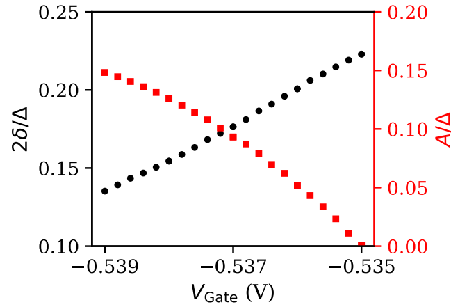
Figure I4. Dependence of the energy gap 2\delta and the splitting A , in units of \Delta , on the gate voltage V_{\text{Gate}} .
