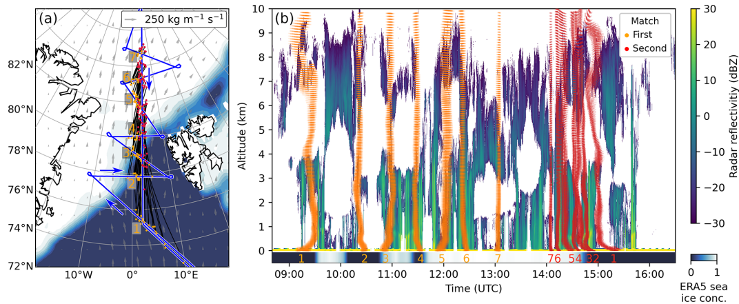
Figure 4. Visualization of quasi-Lagrangian matches for the HALO RF 03 on 13 March 2022. The map in (a) shows the flight track of HALO overlaid on ERA5 data of sea ice concentration and integrated water vapor transport (gray arrows). In (b), a vertical cross section of HAMP radar reflectivity is shown. The first sampling locations (start points) of matches are indicated in both panels by orange dots and the second locations (end points) by red dots. For the map in (a) these start/end points represent altitudes close to the surface and are connected by the trajectories. Number labels in both panels indicate the individual branches of start/end points.
