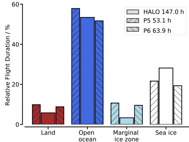
Figure 2. Classification of flight times over specific surface types separated for all aircraft individually.
