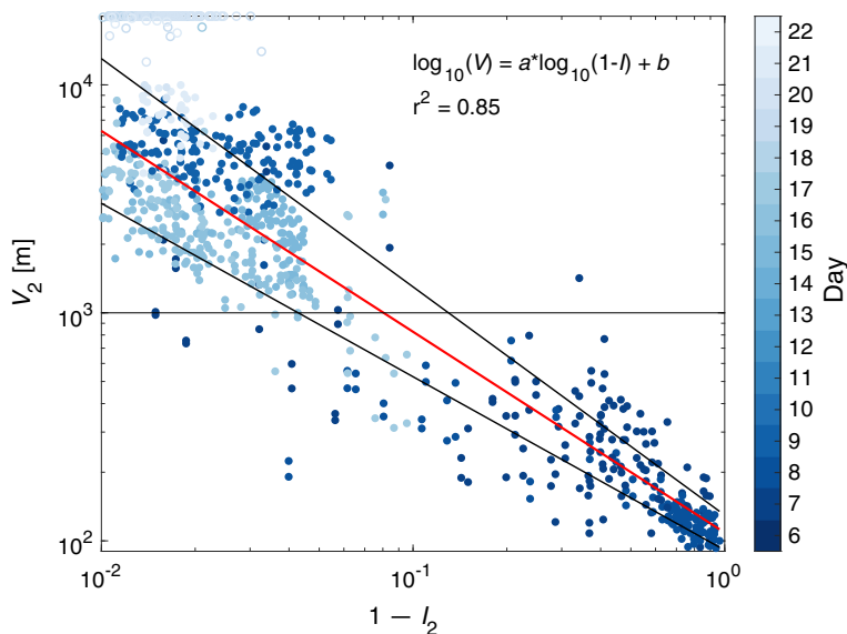
Fig. 10 Regression relating the saturation of the camera pixels (1 minus pixel intensity) at 2.0-m height to the observed visibility measured on both KNMI visibility sensors. The red line is the linear regression of Eq. 7 and the black lines are the 99% confidence intervals. The empty circles indicate data that were excluded from the regression
