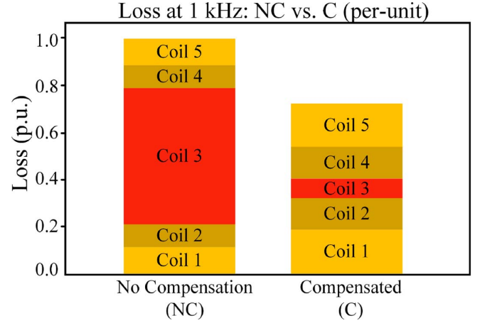
Fig. 10. Comparison of the losses of each coil before and after compensation.
