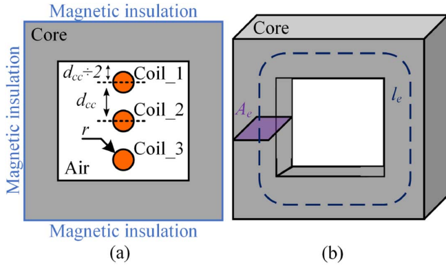
Fig. 1. (a) Simple 2-D problem with three parallel coils inside the core window; (b) 3-D view of a magnetic core illustrating the effective magnetic path length l_e and the effective cross-sectional area A_e .
