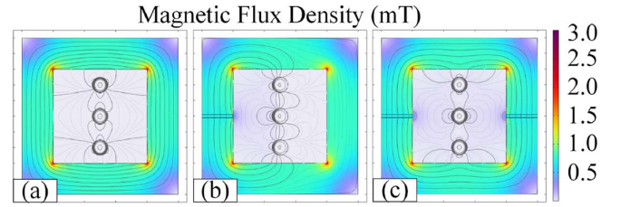
Fig. 6. FEM Simulation results of the impact of air gap in the core: (a) without gap; (b) air gap on one leg; and (c) air gaps on both legs.
