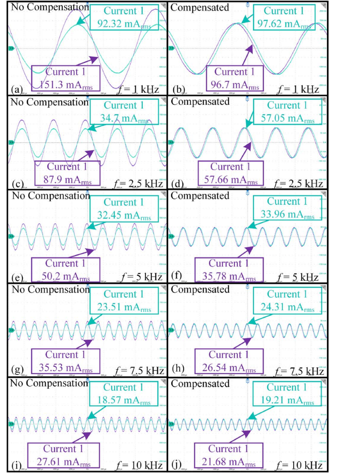
Fig. 16. Experimental results before and after applying compensation toroids at 1, 2.5, 5, 7.5, and 10 kHz.
