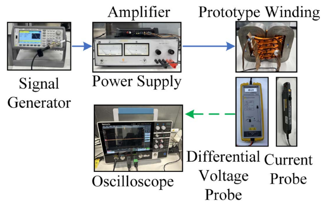
Fig. 13. Test setup block diagram.
