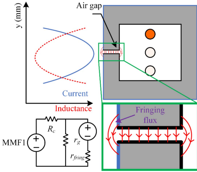
Fig. 4. Equivalent magnetic circuit of a gapped magnetic core considering the fringing effect. The upper and lower coils have higher inductance and lesser current than the inner coil.
