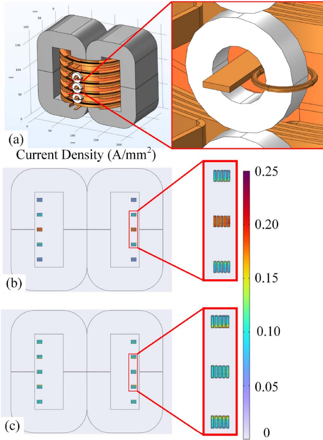
Fig. 9. FEM simulation for the prototype: (a) 3-D model and the compensation toroid; (b) current density ( \text{A/mm}^2 ) over parallel-connected coils around the core before applying the compensation toroids; and (c) impact of applying compensation toroids.
