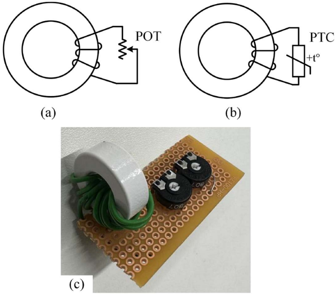
Fig. 14. Compensation toroids using auxiliary winding as fine-tuning method: (a) using a potentiometer; (b) using a positive-temperature-coefficient (PTC) thermistor; and (c) the prototype compensation toroid.
