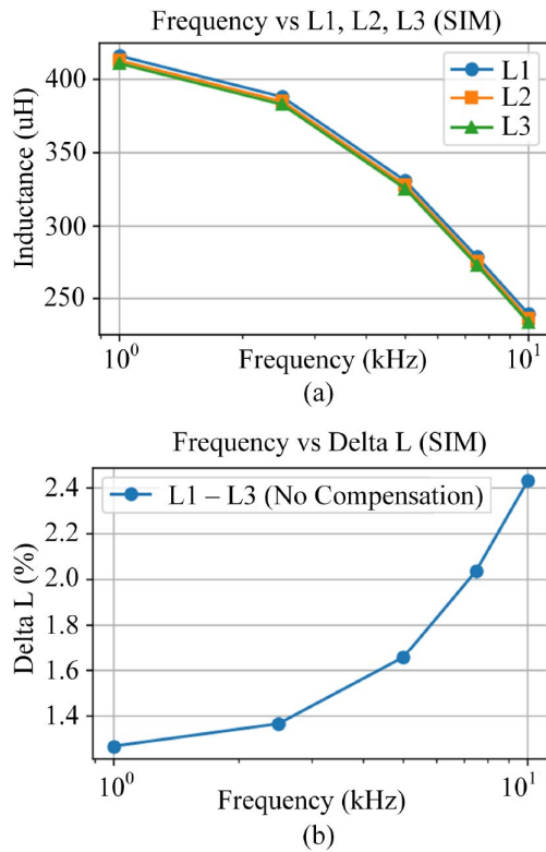
Fig. 17. (a) Changes of the inductances of the coils over frequency; and (b) difference in inductance between coil #1 and coil #3 at different frequencies without compensation. The mismatch increases at higher frequencies, emphasizing the need for frequency-specific compensation.
