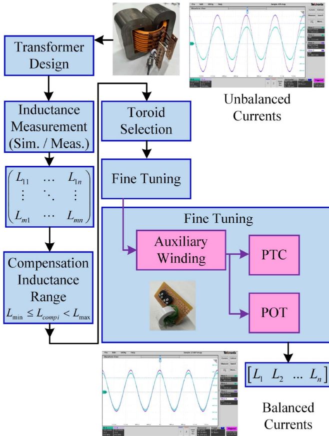
Fig. 15. Flowchart of presented method. The designed transformer might face unbalancing in current distribution. The compensation inductances are designed and fine-tuned to achieve current balancing.
