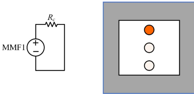
Fig. 2. Equivalent magnetic circuit when coil_1 is excited by a current and other coils are left open circuit ( I = 0 ).
