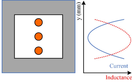
Fig. 3. Current sharing and inductance comparison of parallel coils (disks) of a winding around a nongapped magnetic core. The upper and lower coils have lesser inductance and higher current than the inner coil.
