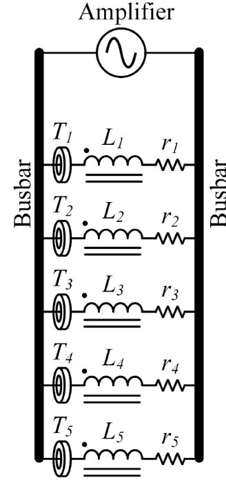
Fig. 8. Proposed method for mitigating current unbalancing in the parallel coils using compensation toroids.
