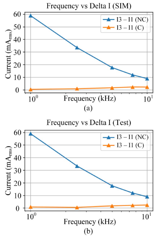
Fig. 18. Simulation versus experimental results: (a) difference between currents of coil #1 and coil #3 at various frequencies with (C) and without compensation (NC); and (b) the same results from experiments. The compensated case maintains minimal imbalance across frequencies, demonstrating the effectiveness of the tuning method.
