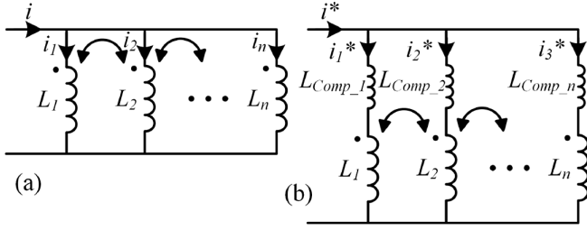
Fig. 7. Parallel coils as parallel connected coupled inductors: (a) without compensation; (b) with the compensation toroids.
