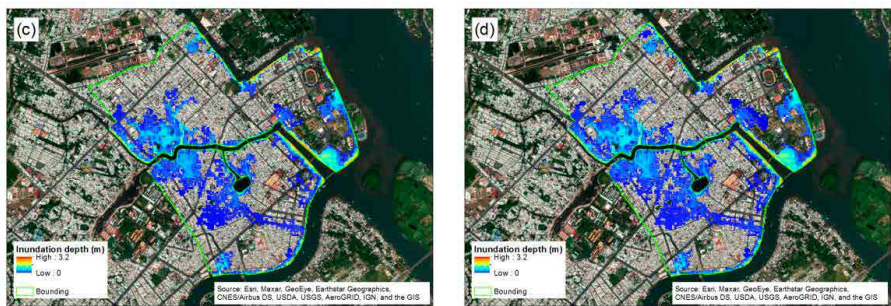
Figure 3.12. Flood hazard maps for 2050 under RCP 4.5 (model scenario #2) corresponding to each return period of water level, (a) 0.5 yr return period, (b) 5 yr return period, (c) 50 yr return period, (d) 100 yr return period
