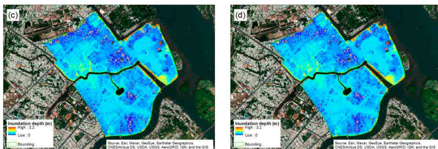
Figure 3.16. Flood hazard maps for 2050 under RCP 8.5 (model scenario #3) corresponding to each return period of water level, (a) 0.5 yr return period, (b) 5 yr return period, (c) 50 yr return period, (d) 100 yr return period
