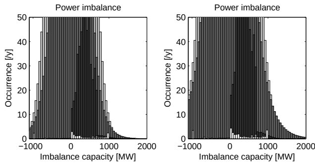
Figure 4.29: Sensitivity analysis: longer time-frame (3GW wind) [73].
