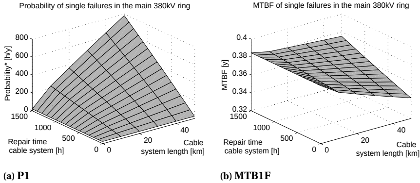
Figure 3.34: (Annualized) probability and MTB1F of single failures in the main 380kV ring.
