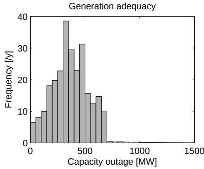
Figure 4.24: Occurrence of generation capacity outages [73].
