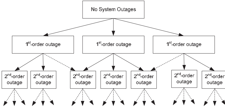
Figure 2.16: State enumeration.
