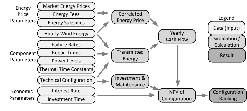
Figure 4.17: Overview of the NPV method [23].
