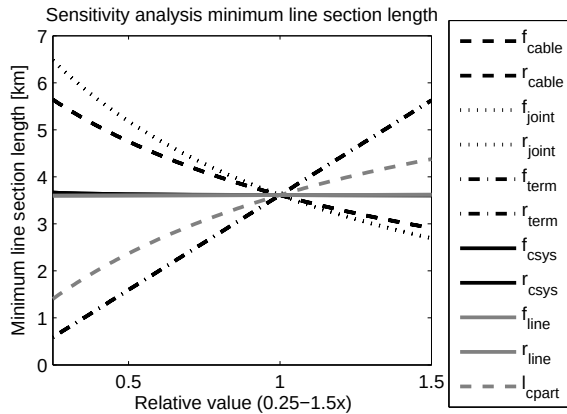
Figure 3.6: Sensitivity of the minimum line section length to input parameter changes. The x-axis shows the relative values of the input parameters (where 1 = the parameters as given in table 3.1 (high estimation)). Lines with the same color and pattern are located below each other.
