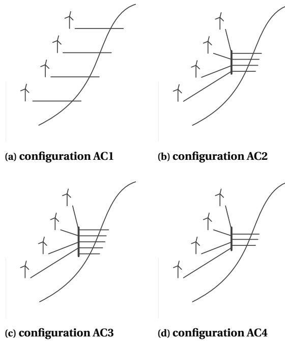
Figure 4.5: Hub-at-sea configurations (AC).
