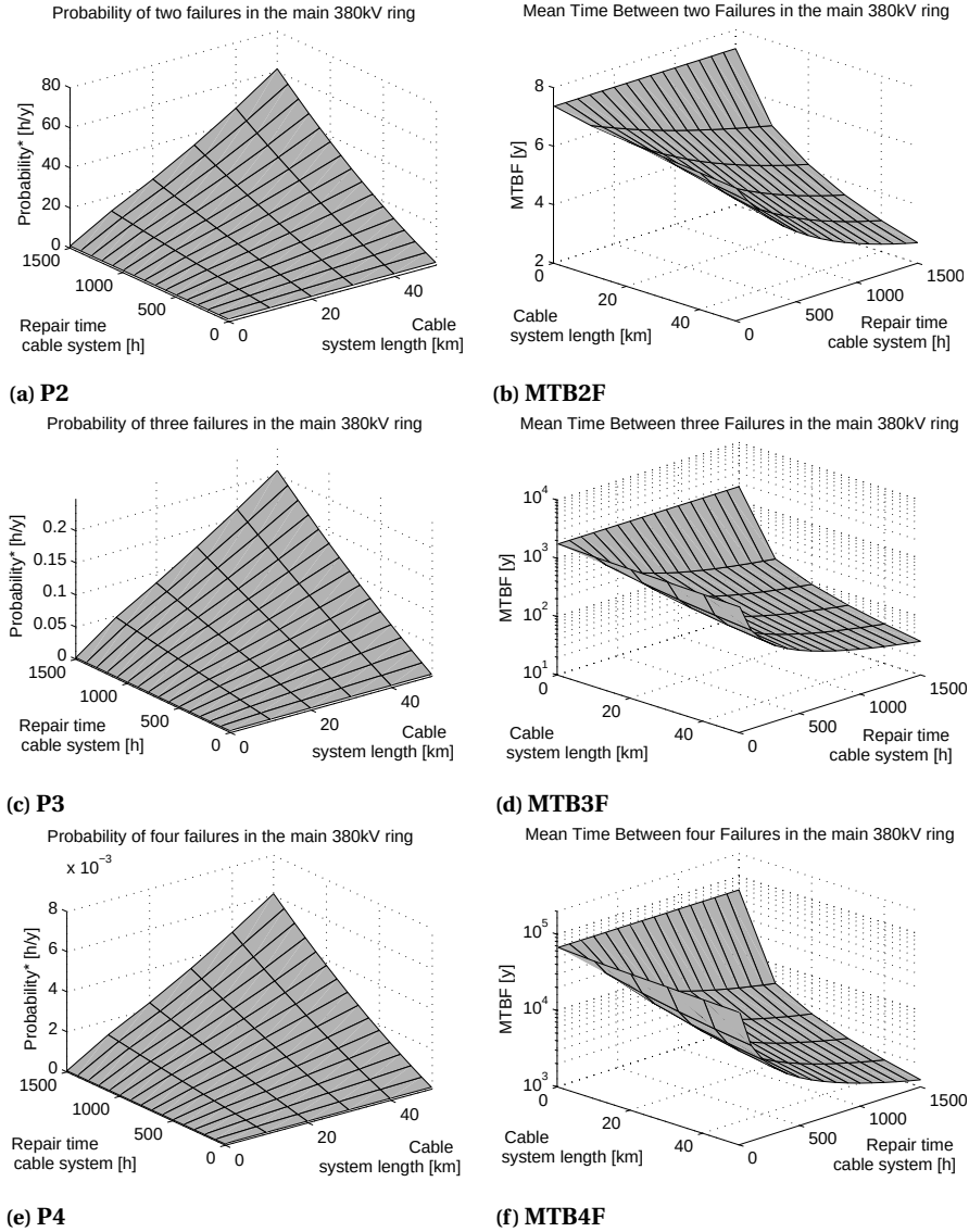
Figure 3.35: (Annualized) probability and MTBF of higher-order failures in the main 380kV ring.
