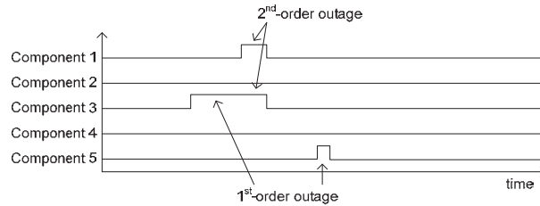
Figure 2.19: Monte-Carlo simulation.
