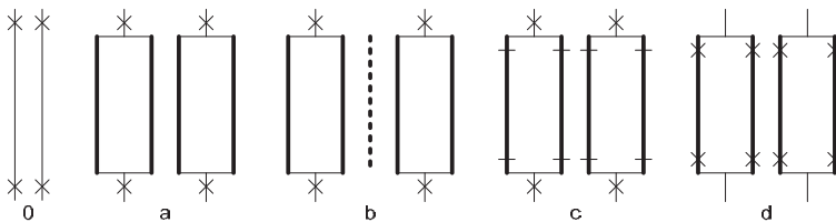
Figure 3.8: Configurations of UGC double circuit. 0 = double overhead line circuit, a = double cable circuit (circuit switching), b = a with additional spare cable, c = double cable circuit with additional disconnectors (circuit switching), d = double cable circuit with additional circuit breakers (cable switching).
