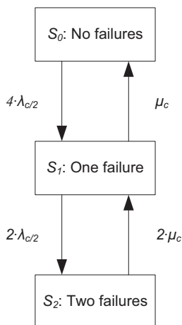
Figure C.12: Markov model of configuration 2a.
