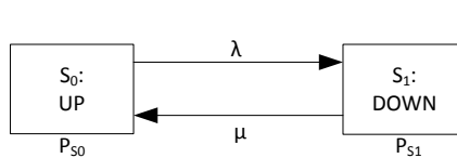
Figure 2.7: Two-state Markov model of a repairable component.
