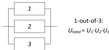
Figure 2.9: Parallel Connection (1-out-of-N).
