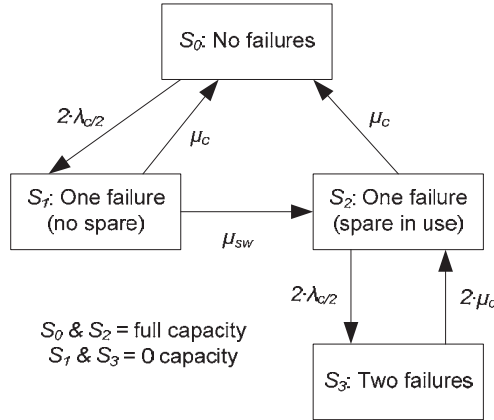
Figure C.8: Markov model of configuration 1b.
