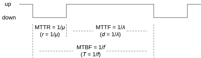
Figure 2.5: Life cycle of a component.
