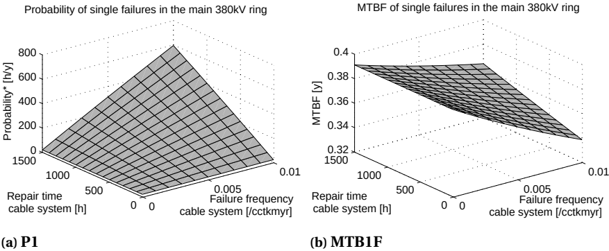
Figure 3.31: (Annualized) probability and MTB1F of single failures in the main 380kV ring.
