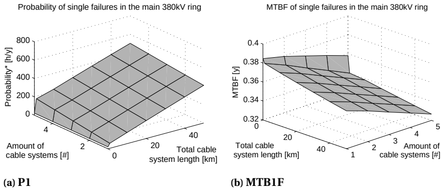
Figure 3.38: (Annualized) probability and MTB1F of single failures in the main 380kV ring.
