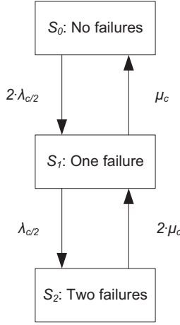
Figure C.10: Markov model of configuration 1d.
