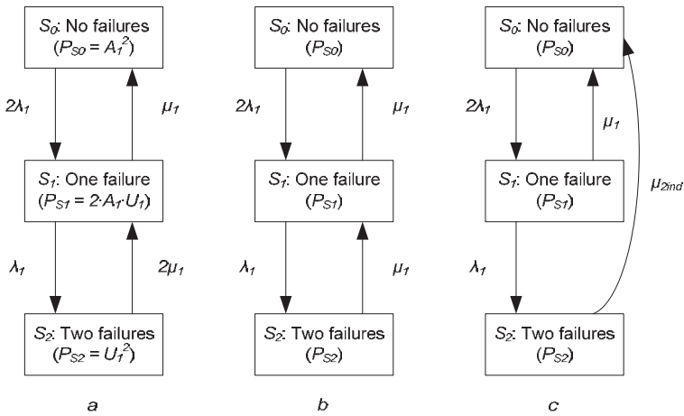
Figure C.3: Markov models for independent double circuit failures. a= independent individual repairs, b=one repair team, c=separate repair processes for independent/dependent failures. None of these represent reality perfectly well. Because of simplicity, model a is preferred.
