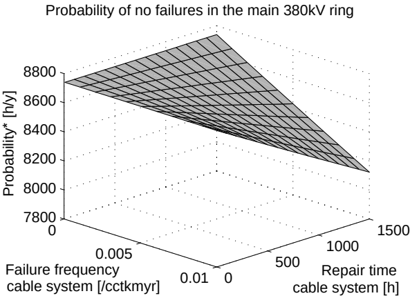
Figure 3.30: (Annualized) probability of no failures in the main 380kV ring. The indicated failure frequency is measured in /cctkm-yr. It is assumed that this value includes the failure frequencies of the joints and terminations as well. For this calculation, one double circuit cable section of 10 km is included in the network.
