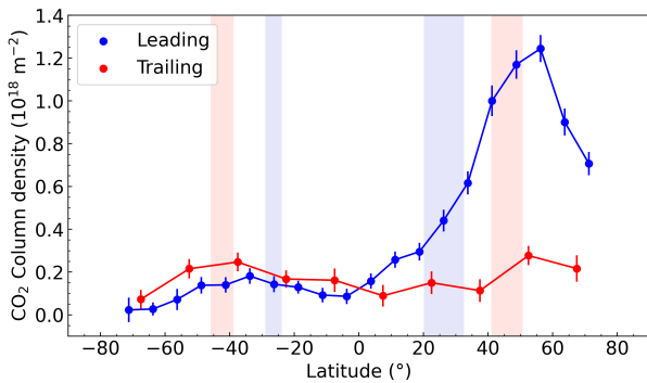
Fig. 2. Variation of CO 2 gas line-of-sight column density with latitude. The blue and red symbols refer to the leading and trailing sides, respectively. The column densities were derived from spectra that were averaged in latitude bins of 7.5^\circ (leading, Fig. B.2) and 15^\circ (trailing). The blue (resp. pink) vertical domains show the latitude range of the OCFBs for the leading and trailing sides, respectively, restricted to longitudes of 10\text{--}130^\circ\text{W} (leading) and 210\text{--}330^\circ\text{W} (trailing).
