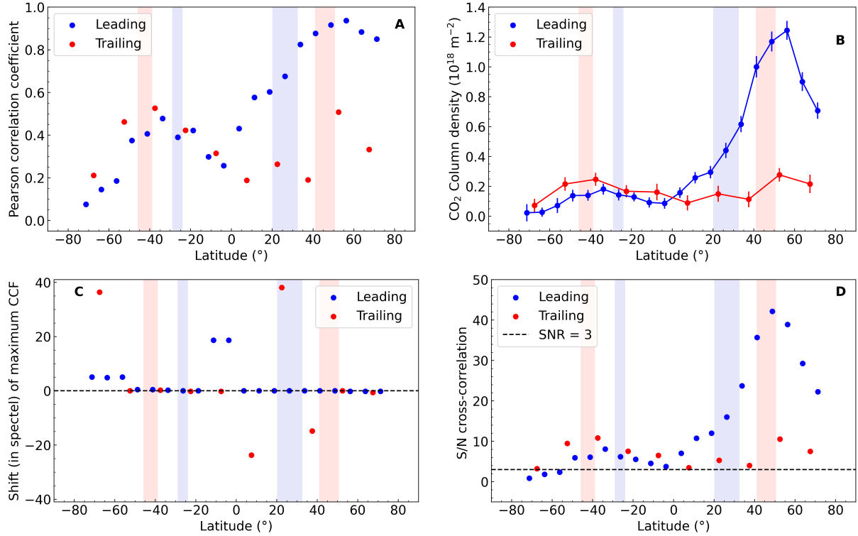
Fig. C.2. Study of 4.22–4.295 \mu\text{m} spectra averaged over latitude bins. A) Pearson correlation coefficient between residual \text{CO}_2 DIFF spectra and a synthetic DIFF spectrum which uses a \text{CO}_2 fluorescence synthetic spectrum at T = 105 K as input. B) \text{CO}_2 line-of-sight column density retrieved from the fit of \text{CO}_2 DIFF spectra. C) shift, in fraction of spectel, of the maximum of the cross-correlation function (CCF) between \text{CO}_2 DIFF spectra and the synthetic DIFF spectrum; secure detection is indicated when the shift is close to zero. D) S/N of the cross-correlation function at shift = 0. The S/N is obtained by computing the \text{CCF}_{\text{noise}} obtained by using as input a simulated noisy spectrum, with the r.m.s deduced from the ERR entry in the Level 3 data cube, and scaled in \sqrt{n} , where n is the number of averaged spaxels ( \text{S/N} = \text{CCF}/\text{CCF}_{\text{noise}} at shift = 0). In all plots, blue and red symbols correspond to the leading and trailing sides, respectively. The blue (resp. pink) vertical domains show the latitude range of the open-closed field-line boundaries for the leading and trailing sides, respectively, restricted to longitudes of 10–130° W (leading) and 210–330° W (trailing).
