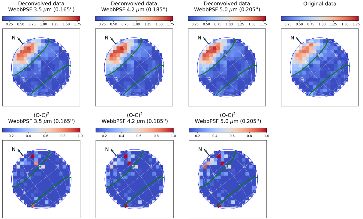
Fig. M.1. PSF deconvolution. Top: deconvolved CO 2 -gas maps (leading hemisphere) obtained with the AIDA algorithm using NIRSpec PSFs calculated with WebbPSF at 3.5 \mu\text{m} (FWHM = 0.165"), 4.2 \mu\text{m} (FWHM = 0.185") and 5 \mu\text{m} (FWHM = 0.205"). Bottom: residuals of the deconvolution for each calculated PSF; plotted are (O - C)^2 , where O is the original CO 2 column-density map (leading hemisphere, top-right plot), and C is the convolution of the deconvolved O map. Color bars are in unit of 10^{18} \text{ m}^{-2} .
