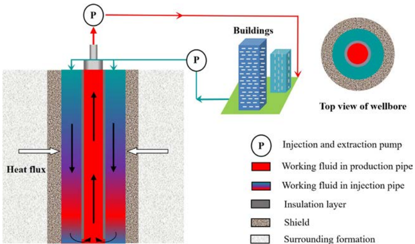
Fig. 16 Schematic diagram of geothermal heating from an abandoned oil well.
