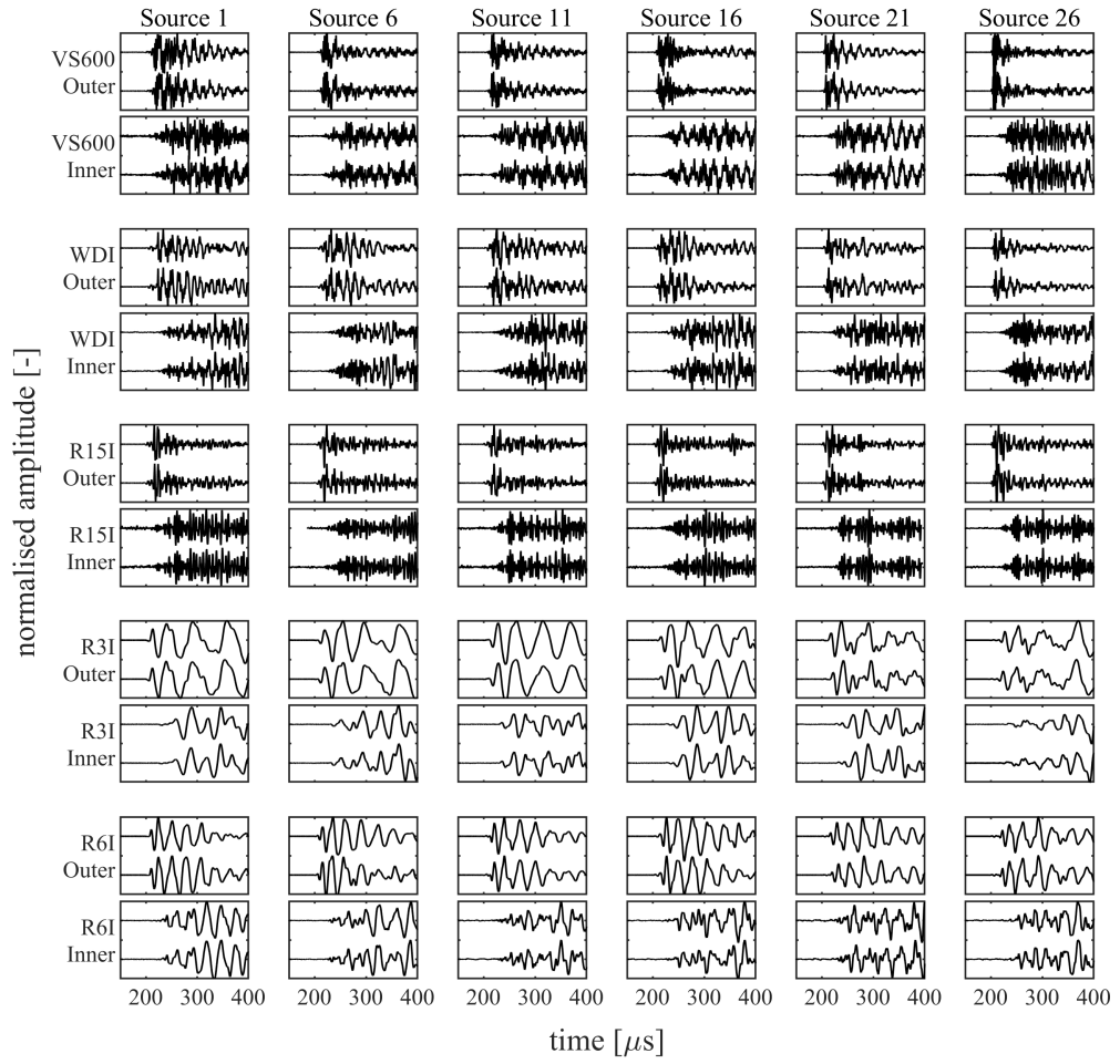
Figure 2.4: Overview of recorded waveforms for several outer raceway sources. Each block depicts a 250 \mu s sample of two waveforms that have been normalised with their respective peak amplitudes.
