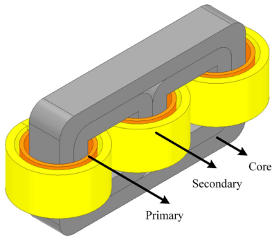
FIGURE 10. 3D view of the MMC-SST MFT.
