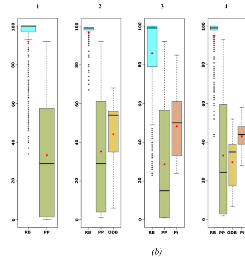
Fig. 6. Measures selection analysis for four strategies, with the objectives of cost minimisation and (a) flood risk reduction, (b) total benefits maximisation. With RB: rain barrels, PP: pervious pavements, ODB: open detention basins, Pi: pipes.
