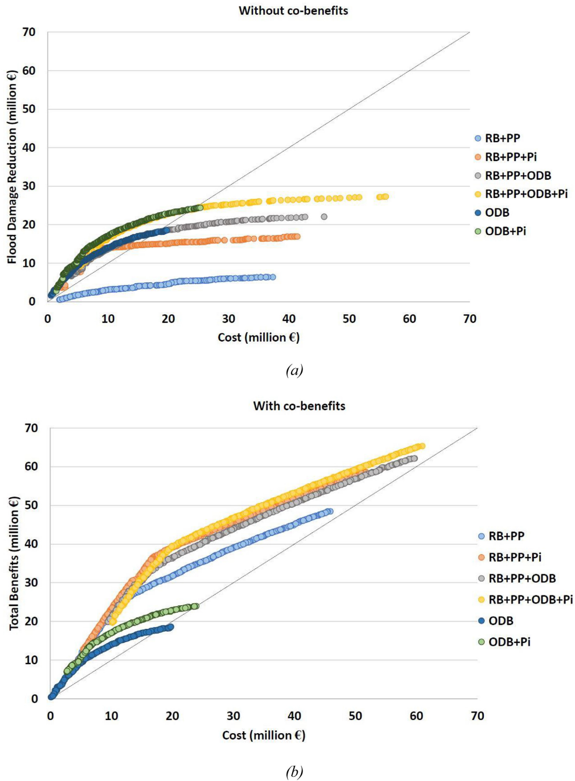
Fig. 4. Pareto fronts obtained for the six strategies selected with (a) cost minimisation and flood risk reduction maximisation as objectives (b) cost minimisation and total benefits maximisation as objectives (grey line: costs = benefits).
