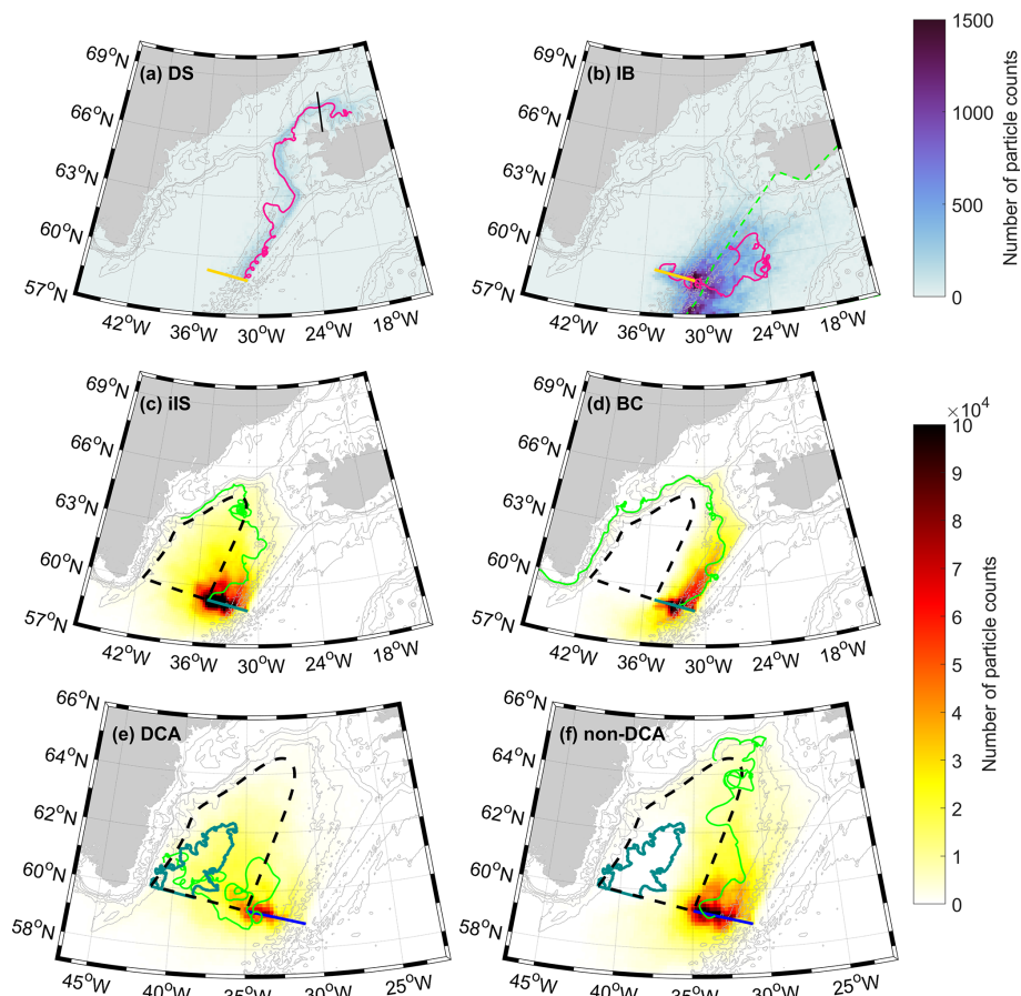
Figure 4. Particle density maps of particles released at the OSNAP IC moorings. Particle density distribution for (a) Denmark Strait particles and (b) Iceland Basin particles. The pink line marks an example particle track and the orange line the release line. Dashed black line in (a) and green dashed line in (b) geographically mark the selection criterion for DS and IB respectively. Particle density distribution for (c) interior and (d) boundary current with example particle tracks (green) and interior Irminger Sea definition (dashed line); release line is marked in greyish blue. (e) DCA particles and (f) non-DCA particles with example particle tracks (green), contours defining the interior Irminger Sea (dashed line) and the DCA (blue); dark blue line marks the particle release line. Note the different colorbar limits are used for (a, b) compared to (c–f) because of the large difference in particle amount per grid box.
