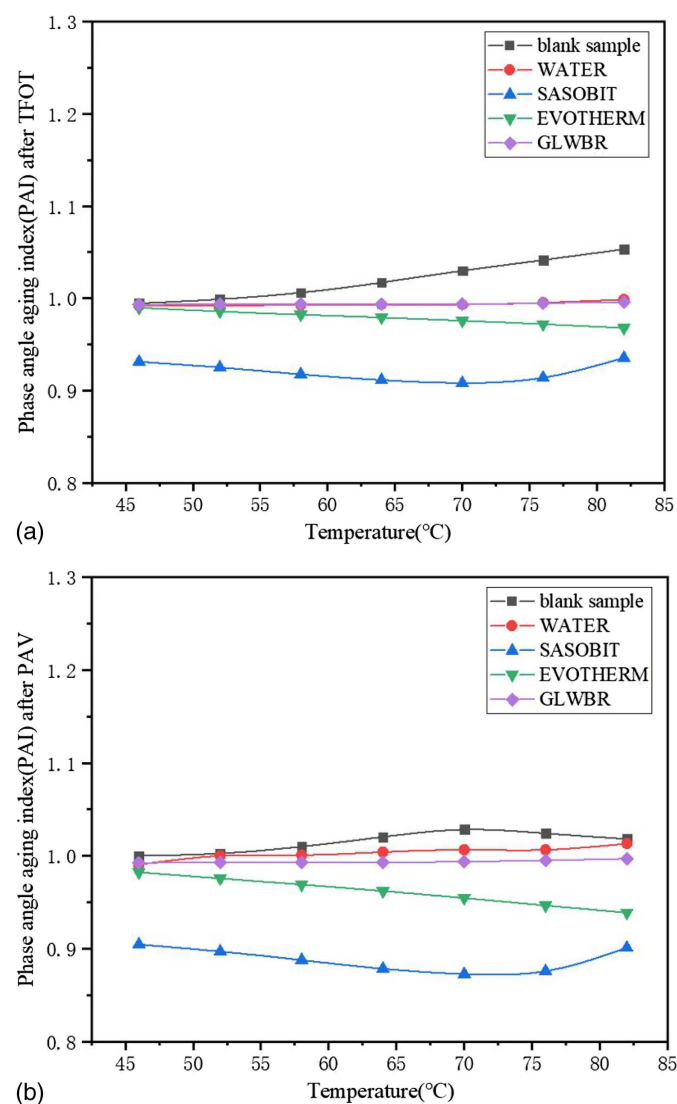
Fig. 13. PAI values of different warm-mix HVMAs after: (a) TFOT; and (b) PAV.
