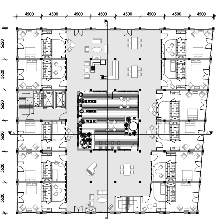
First floor 1:400
