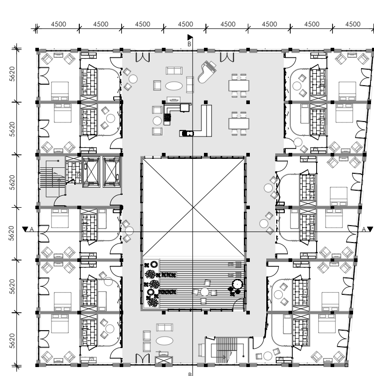
Second floor 1:400
