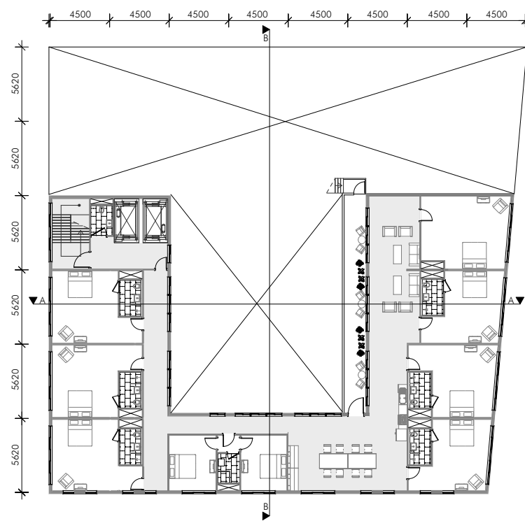
Fifth floor 1:400
