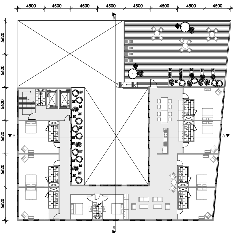
Fourth floor 1:400
