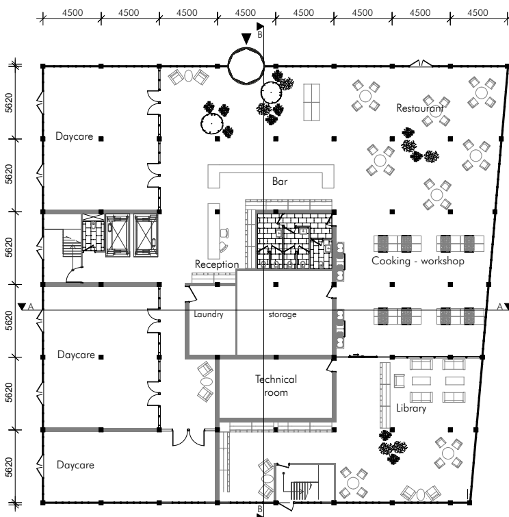
Ground floor 1:400
