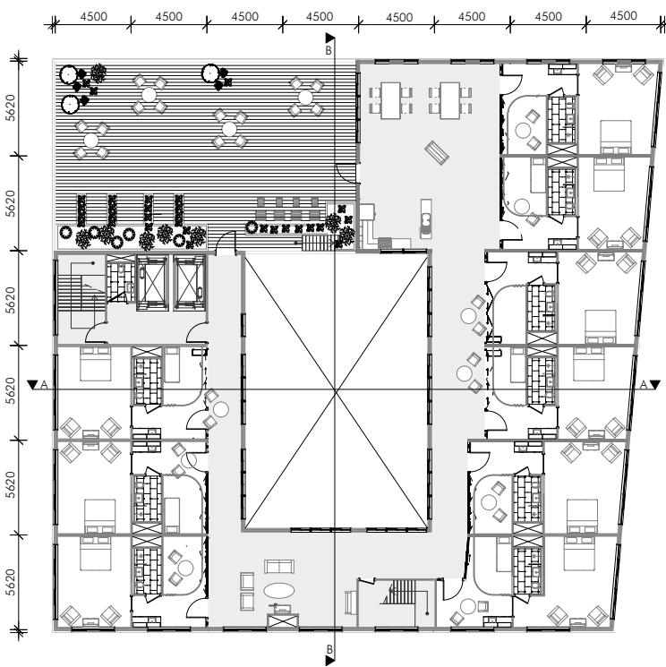
Third floor 1:400
