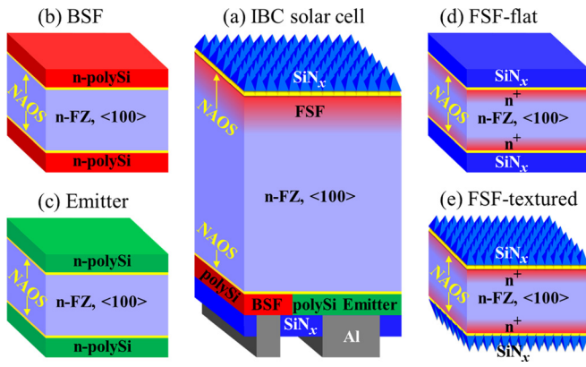
FIG. 1. (a) Schematic illustration of the front-textured interdigitated back contact (IBC) silicon solar cell with ion-implanted LP-CVD polycrystalline silicon (polySi) based tunnel oxide passivating contacts (TOPCon) as both emitter and back surface field (BSF). At the front side of the cell is the ion-implanted crystalline silicon (c-Si) as the front surface field (FSF), which is passivated by nitric acid oxidation of silicon (NAOS) and \text{SiN}_x . Symmetrical test structures are also sketched for (b) polySi BSF, (c) polySi emitter, and homojunction P-implanted (d) flat FSF and (f) textured FSF, which are passivated by nitric acid oxidation of silicon (NAOS)/ \text{SiN}_x .
