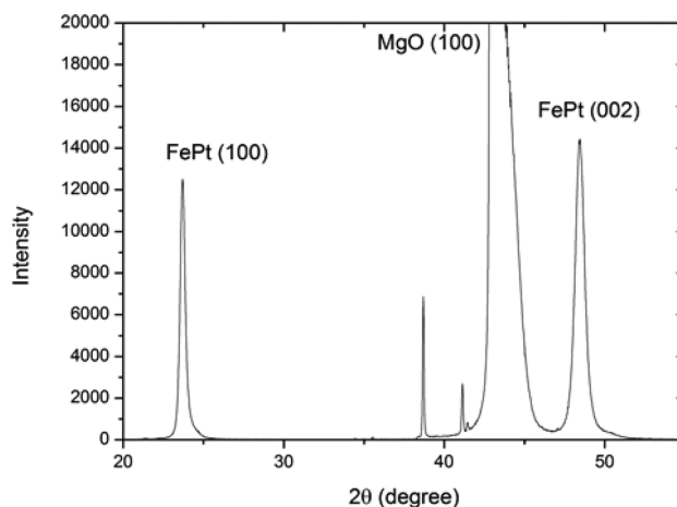
FIG. 1. X-ray diffraction of the MBE-grown FePt films.
