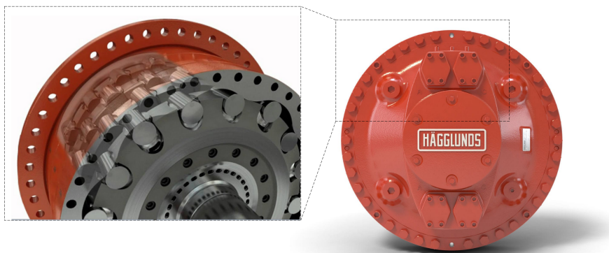
Figure 2.4: The basic layout of the Hagglunds CB radial piston. Several versions with varying power, volumetric output and operating pressures are available.
