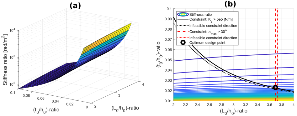
Figure 8.12: (a) Parametric analysis on the stiffness ratio for h_0 = 1(\text{m}) and (b) an example of an optimization strategy.
