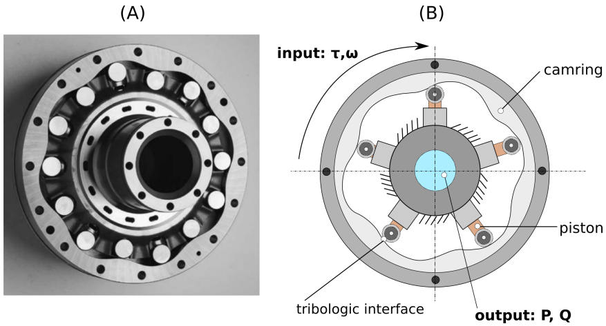
Figure 2.5: (Left) The basic lay-out of a radial piston pump utilizing a camring to obtain a higher gear ratio. (Right) The basic input and output for a radial piston pump, specifically defining the crucial tribology interface.
