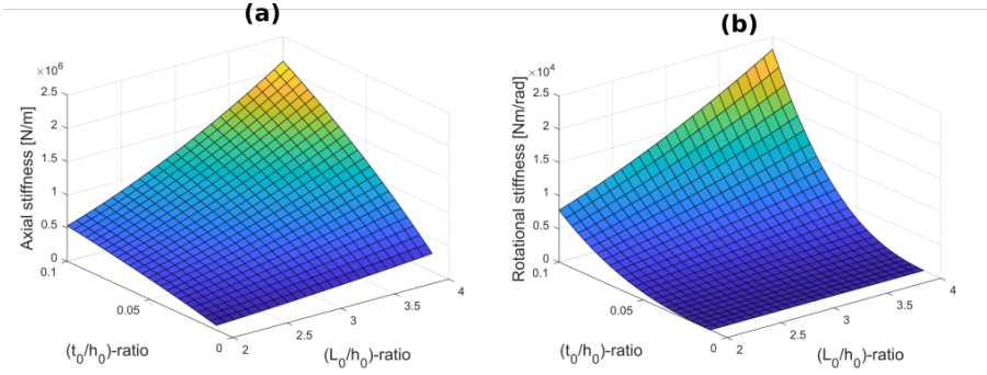
Figure 8.11: Parametric analysis on the (a) axial and (b) rotation stiffness for h_0 = 1(\text{m}) .
