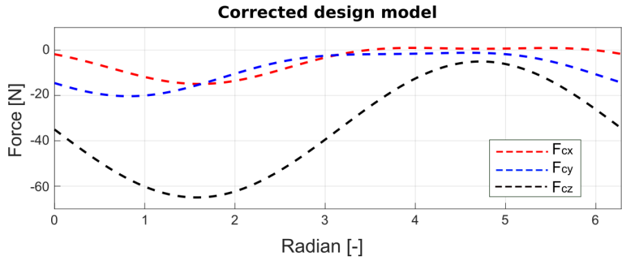
Figure 9.19: Corrected model results that determine the expected shear forces. This model assumes also the corrected friction coefficient found for the proposed material combination.
