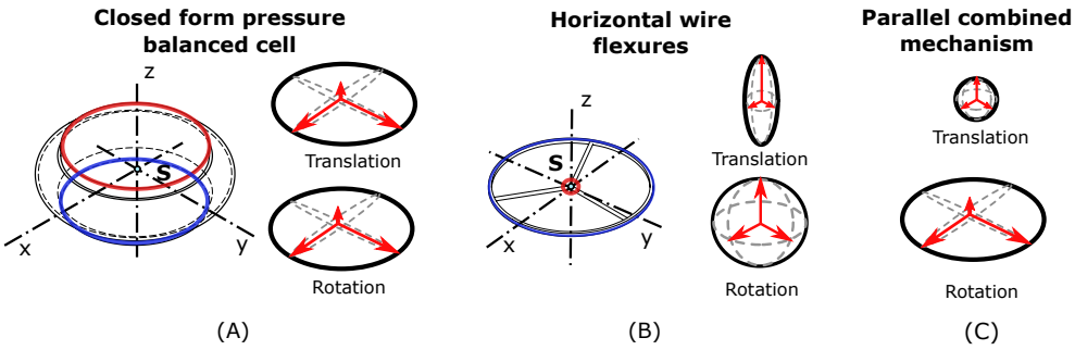
Figure 9.3: Compliance ellipsoids for the axi-symmetric topology of the closed form pressure balanced joint (A), the tension constraining wire-set (B) and a parallel combination of the two (C).
