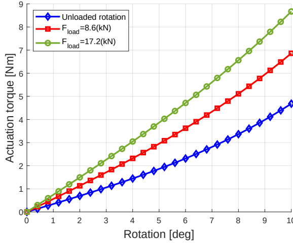
Figure 8.14: Effect of varying axial loads on the rotation stiffness, simulated for (L_0/h_0) = 3 , (t_0/h_0) = 0.05 and h_0 = 1 \text{ (m)} .
