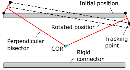
Figure 8.9: Schematic construction of the instantaneous COR.
