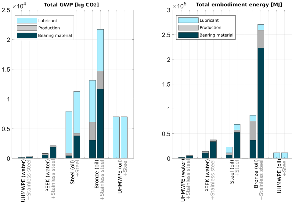
Figure 3.12: Total GWP and embodied energy for the 5 material/lubricant combinations analyzed in the case study. In all cases, both the worst and best case material scenario's (recycled or virgin) have been presented. The total GWP for water lubricated UHMWPE-stainless steel is 191.44 and 360.72 kg CO 2 , and the total embodied energy equals 3335.72 and 6920.33 MJ respectively.
