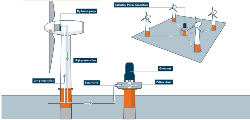
Figure 2.2: The basic lay-out of the Delft offshore Turbine wind farm. Several wind turbines with each an hydraulic pump are connected to a single large generator through a pelton wheel.
