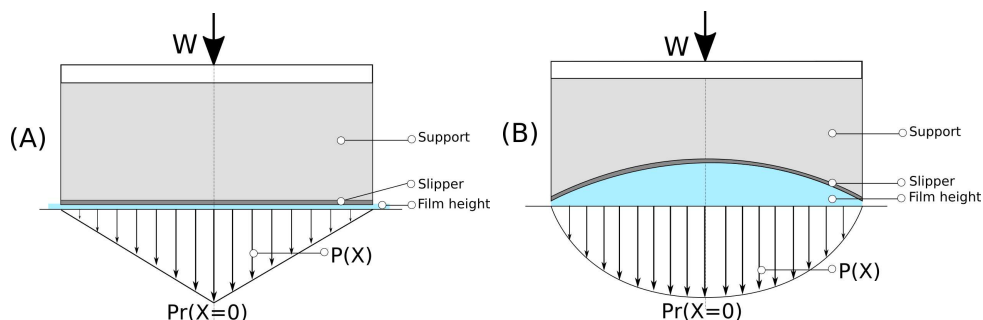
Figure 5.1: (A) An 'infinitely long' high stiffness parallel slider on a flat running track. (B) The same slider with a compliant support. The deformation of the support influences the obtained pressure profile.
