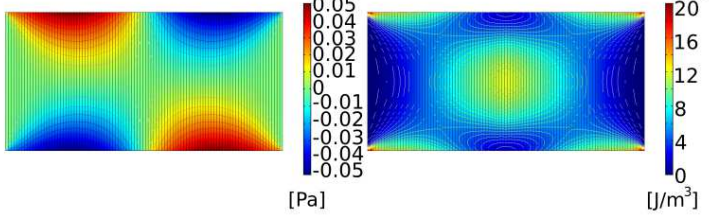
Figure 5.11: Distribution of shear stress \sigma_{xy} and strain energy density W for different discretised supports. Note that all deformations are scaled to 0, and the range of both parameters has been made equal.
