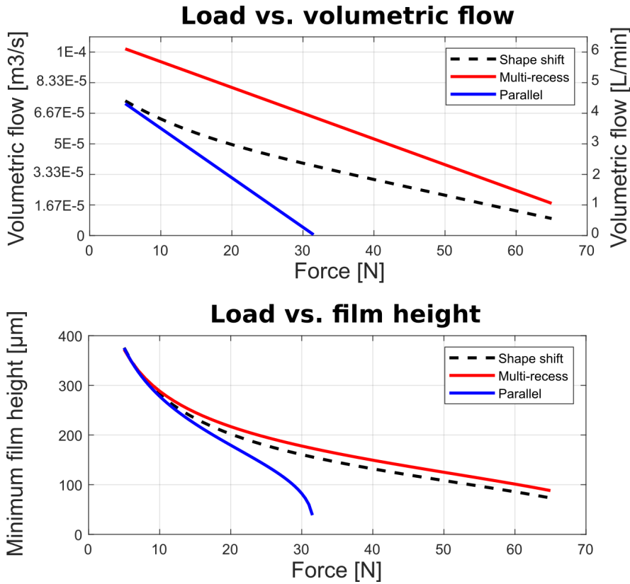
Figure 9.11: The performance of the shape shifting slipper in comparison to its rigid parallel and multi-recess counterparts. The performance is expressed through the volumetric flow vs. load and minimum film height vs. load. The key shape shifting characteristic is clearly visible in the volumetric flow comparison, where the trendline modes from the parallel comparison to its multi-recess counterpart.
