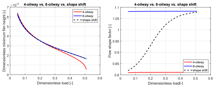
Figure 6.14: The 4-groove vs. 8-groove vs. its shape shifting variant. Both the minimum film height of the bearings as well as the flow shape factors are given for an operation range varying one order of magnitude.
