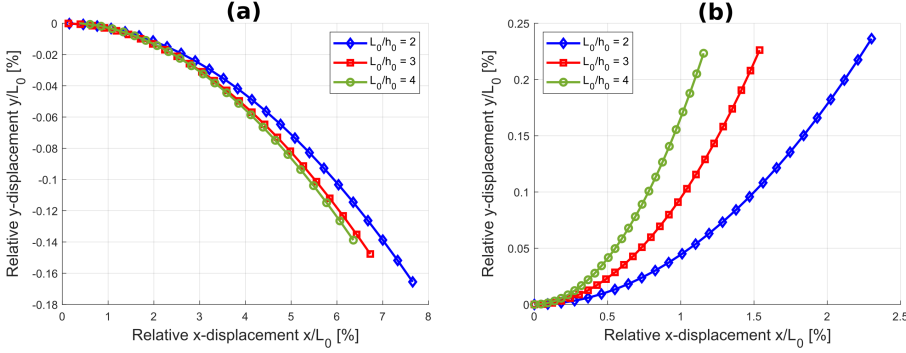
Figure 8.10: Normalized displacement of (a) the COR and (b) the midpoint (x_3, y_3) during a 5^\circ anti-clockwise rotation, simulated for (t_0/h_0) = 0.05 and h_0 = 1(\text{m}) .
