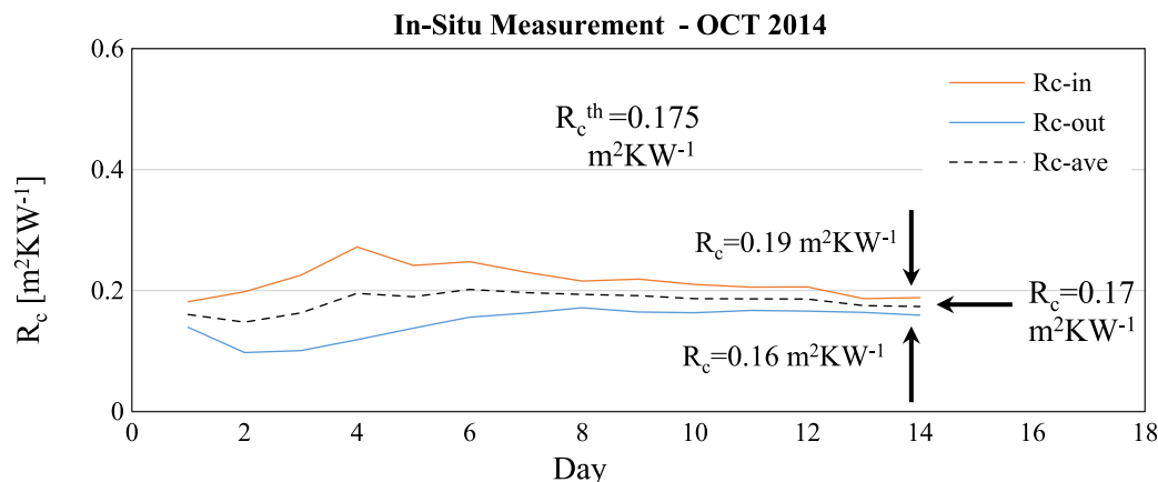
Fig. 12. R_c -value measurements from case study 2: two different R_c -values are obtained, fulfilling the criteria of ISO 9869. Location: The Hague, the Netherlands, Oct 2014.
