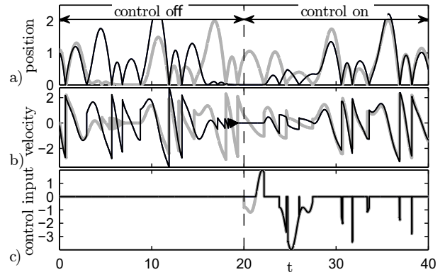
Fig. 3. a,b): Solutions \mathbf{x}(t) and \mathbf{y}(t) and control inputs \tau_x, \tau_y of the 1-DOF mechanical impact oscillators for \mathbf{x} -system in black and for \mathbf{y} -system in grey, respectively. Control inputs are switched on at t = 20 .
