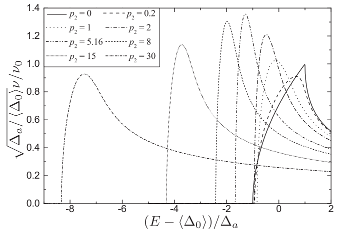
FIG. 6. Density of states vs energy in an anisotropic superconductor containing pairing-potential impurities with a small parameter \mathcal{E}_0 : \mathcal{E}_0 = 0.025|f_{10}^{(2)}|^2\Delta_a , |f_{10}^{(2)}|^2 = 0.1 .
