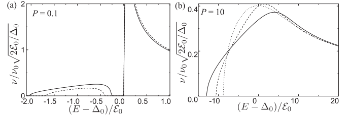
FIG. 2. Density of states vs energy in a superconductor containing either impurities with a local gap suppression [solid line, Eq. (36) with the upper signs] or magnetic impurities with randomly oriented spins [dashed line, Eq. (50)], and the density of states in the universal limit [dotted line in graph (b), Eq. (38)]. The additional shift -P of the gap edge, appearing in Eqs. (36) and (38), is compensated via a positive translation of the corresponding curves by P\xi_0 in graph (b).
