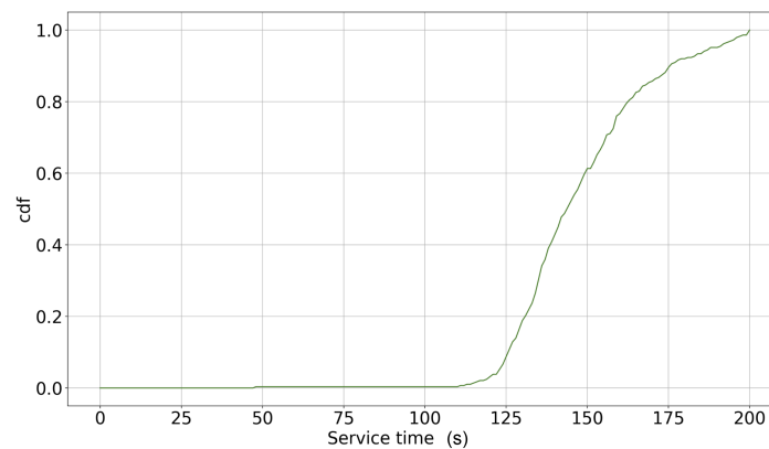
Figure 13. Service time cdf, G(x) .
