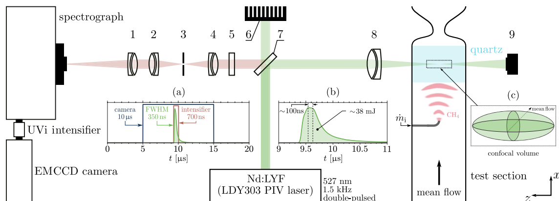
Figure 1. Schematic of the experimental setup. The main components of the Raman system are: (1) achromatic doublet lens ( \varnothing = 25.4 mm, f = 100 mm), (2) achromatic doublet lens ( \varnothing = 25.4 mm, f = 50 mm), (3) mounted pinhole ( \varnothing = 25.4 mm, 25 \mu\text{m} ), (4) achromatic doublet lens ( \varnothing = 25.4 mm, f = 50 mm), (5) 532 nm single-notch filter ( \varnothing = 25.4 mm), (6) beam trap, (7) long-pass 532 nm dichroic beamsplitter ( \varnothing = 25.4 mm), (8) achromatic doublet lens ( \varnothing = 50.8 mm, f = 100 mm), (9) photodiode (PD) detector. Also included: (a) timings of the camera-intensifier-laser system, (b) representative energy time history for a combined two-beam pulsed delivery, and (c) confocal volume schematic (oblate ellipsoid). Dimensions not to scale.
