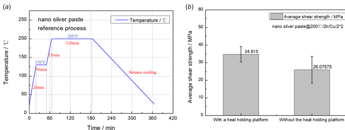
Fig. 5 (a) Reference temperature curve for sintering process and (b) result of the comparison of with or without insulation platform during the reference process
