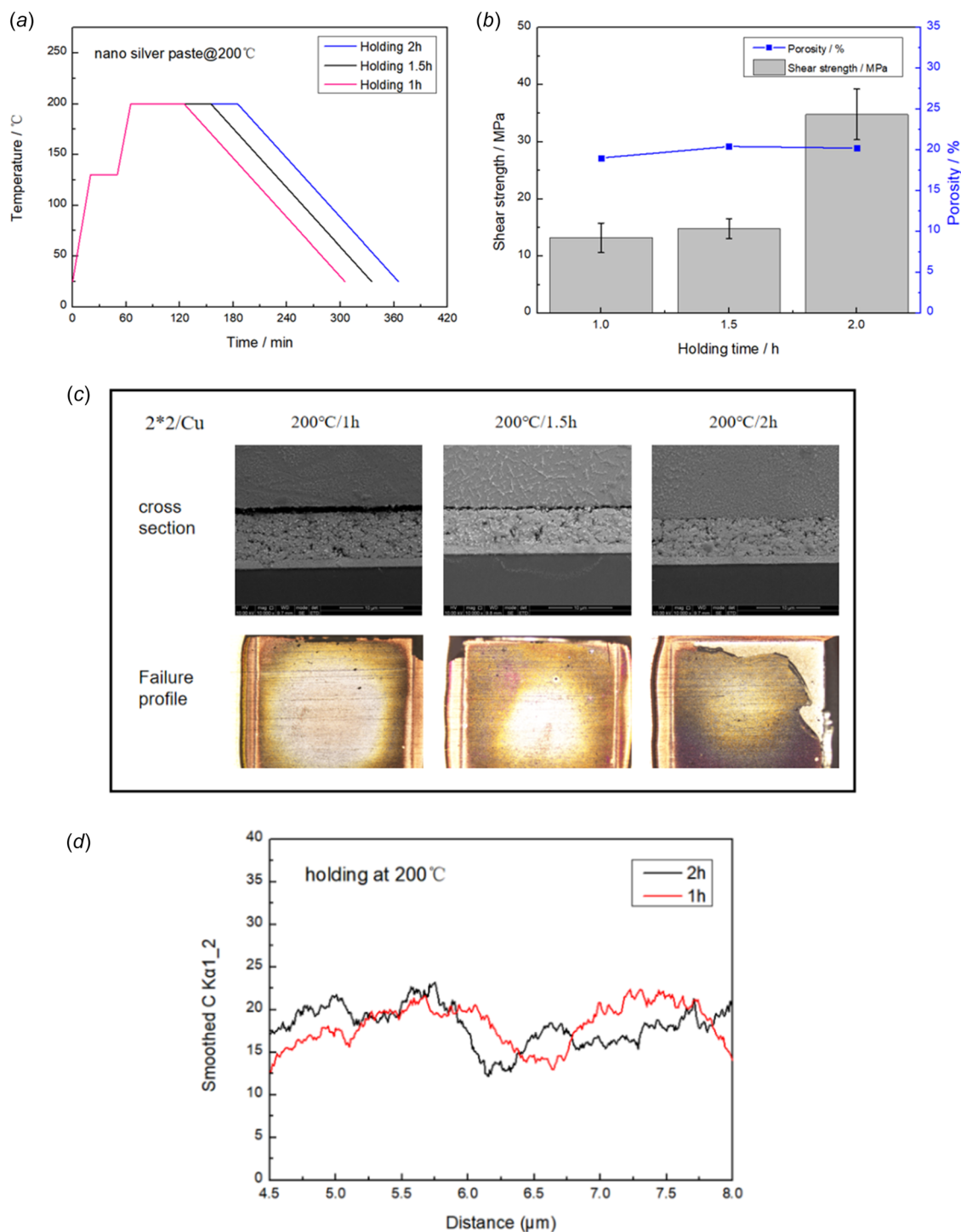
Fig. 8 (a) Process curve under different holding time, (b) results of shear test and porosity analysis, (c) micro-structure analysis after holding 1 h, 1.5 h, 2 h, and (d) EDS analysis of C content after holding at 1 h, 2 h
