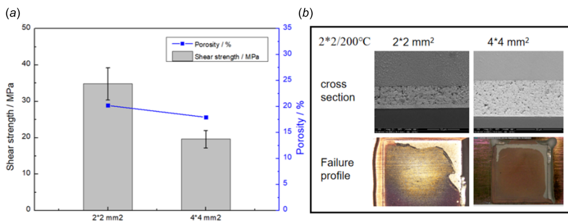
Fig. 10 Results of (a) shear test and porosity analysis and (b) microstructure analysis on different chip size
