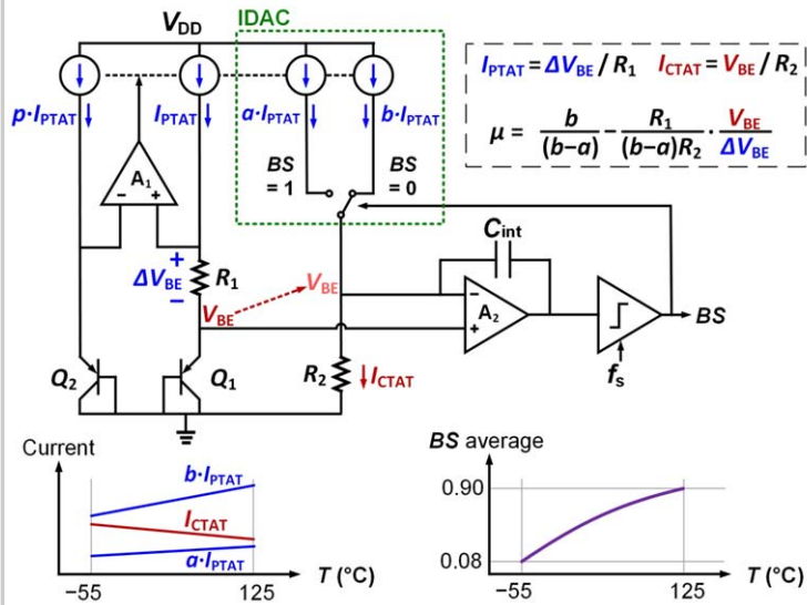
Figure 23.7.1: Operating principle of the proposed BJT sensor (top), and the current signals and bitstream average plotted over temperature (bottom).
