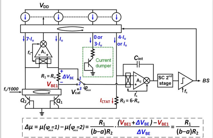
Figure 23.7.2: Simplified schematic of the proposed sensor (top), and the expression used when applying resistor-ratio calibration (bottom).
